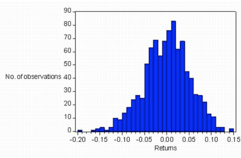
Figure 6. Returns distribution experiment 1 (torus network)
