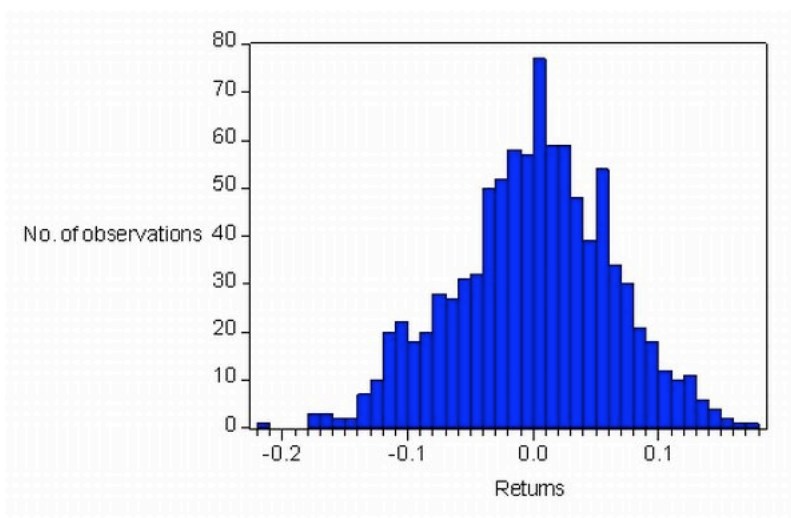
Figure 10. Returns distribution experiment 2 (scale free network)
