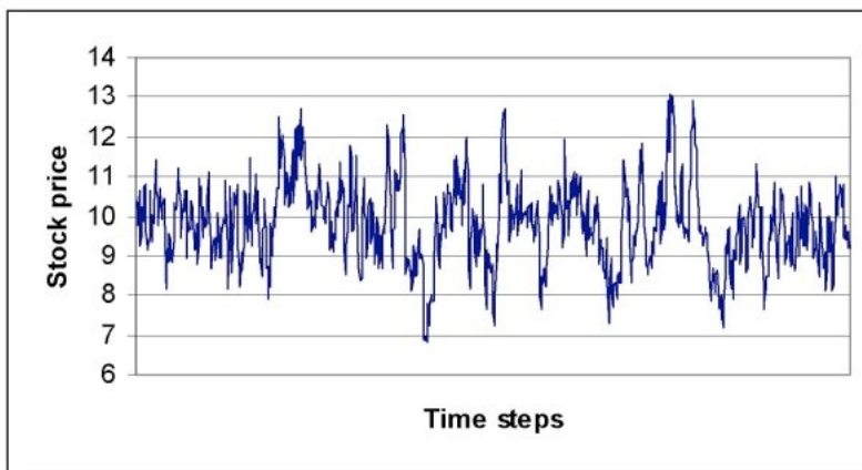
Figure 8. Price time series experiment 2 (scale free network)
