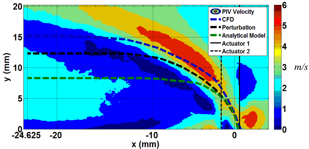
Figure 84 PIV validation of predicted jet centerline trajectories with PIV for R = 2.4 , s = 4.5b , \phi = 0^\circ
