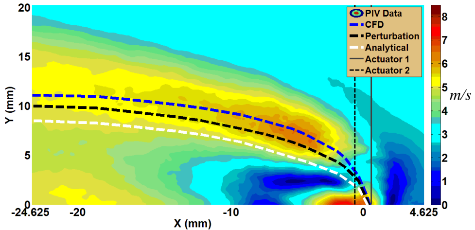
Figure 91 Model validation and flow field analysis for phasing effects \phi = -120^\circ
