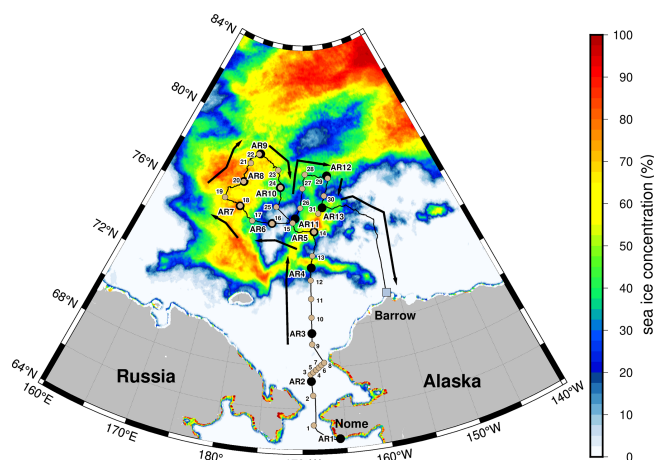
Figure 1. Cruise track (thin black lines) of ARA07B with aerosol- (black circles; sample ID: AR1–AR13) and seawater-sampling (light-brown circles; sample ID: 1–31) locations. Sampling stations were superimposed onto the mean sea ice concentration derived from Advanced Microwave Scanning Radiometer (AMSR) 2 data for August 2016 (Spren et al., 2008). Each aerosol-sampling start point represents the end of the previous sampling period. Thick black arrows indicate the moving direction of the ship.
