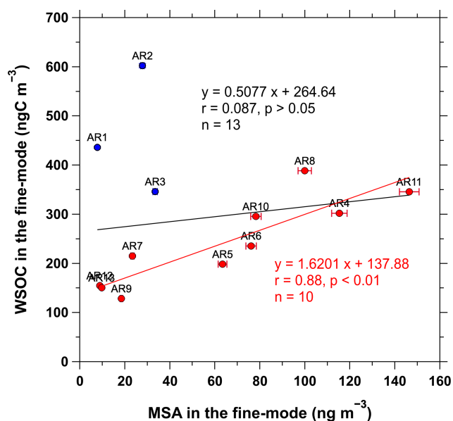
Figure 5. Relationship between WSOC ( \text{ngC m}^{-3} ) and MSA ( \text{ng m}^{-3} ) in the fine-mode aerosols ( D < 2.5 \mu\text{m} ) collected during the cruise. The solid blue and red circles indicate the samples collected from the coastal and sea-ice-covered areas, respectively. The black and red lines indicate the correlations between WSOC and MSA for all samples collected during the cruise and for the aerosol samples collected in the sea-ice-covered areas of the western Arctic Ocean, respectively.
