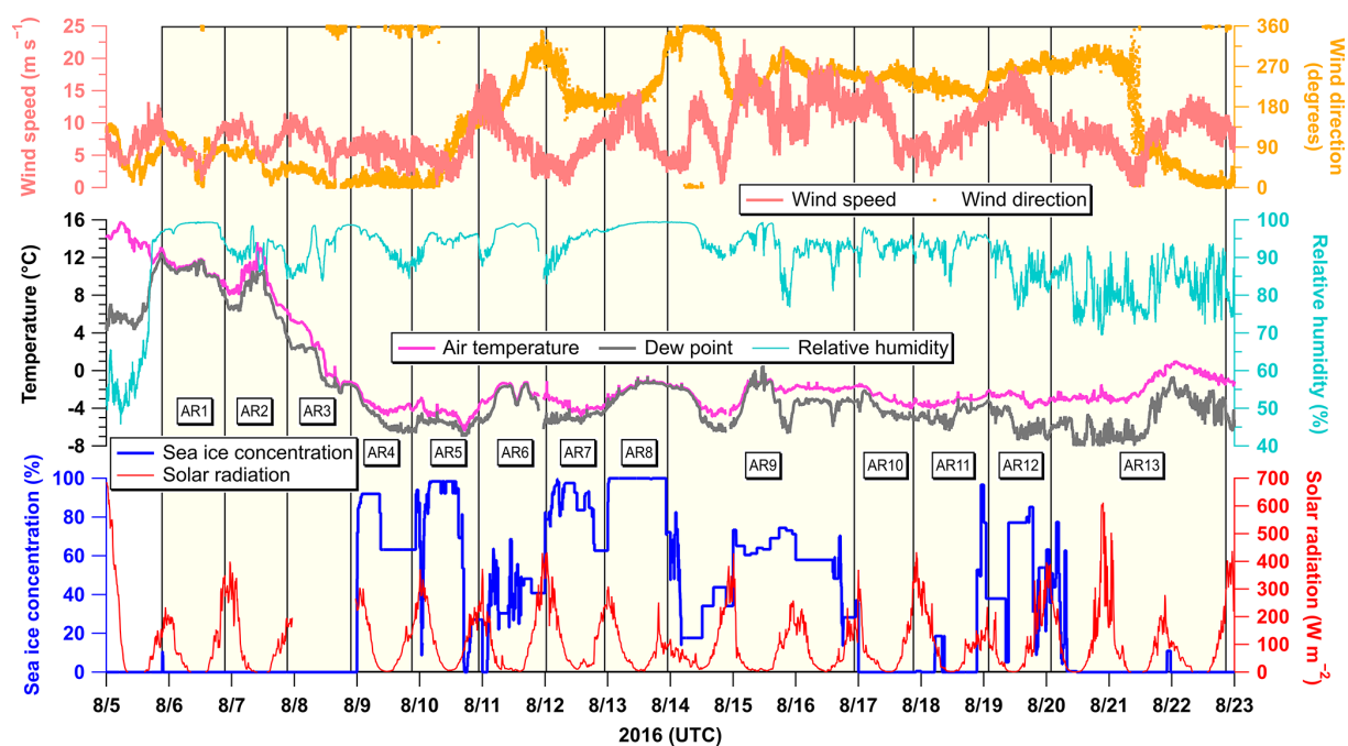
Figure 3. Temporal variations of meteorological variables, including wind speed ( \text{m s}^{-1} ), wind direction (degrees), air temperature ( ^{\circ}\text{C} ), dew point ( ^{\circ}\text{C} ), relative humidity (%), solar radiation ( \text{W m}^{-2} ), and sea ice concentration (%) along the ship's track during the cruise. The hatched yellow area indicates the sampling duration of each aerosol sample (AR1–AR13). Solar radiation was not recorded from 23:20 UTC on 7 August to 23:10 UTC on 8 August due to equipment malfunction. Sea ice concentration represents the percentage of an area covered with sea ice at the ship's location within a 3.125 \text{ km} \times 3.125 \text{ km} grid derived from AMSR 2 sea ice concentration daily data (Spreen et al., 2008).
