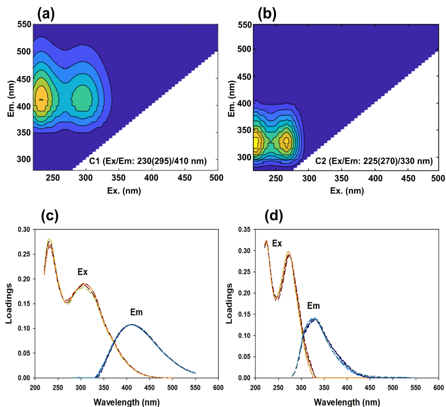
Figure 6. (a, b) Fluorescence EEM contour plots of the two fluorescent components C1 and C2 identified using EEM-PARAFAC for the fine-mode aerosols collected over the western Arctic Ocean during the summer of 2016. (c, d) The loading plots of C1 and C2 showing the split-half graphs.
