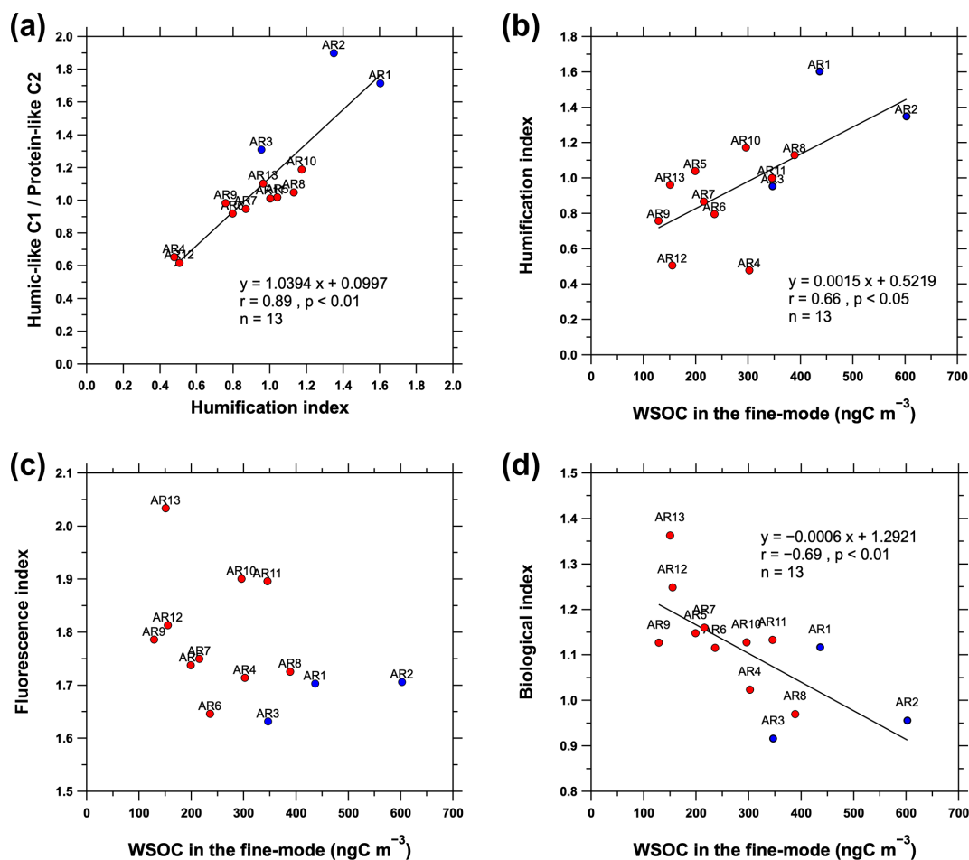
Figure 8. (a) Relationship between the fluorescence intensity ratio of the humic-like C1 / protein-like C2 with humification index (HIX). Relationships between WSOC concentration in the fine-mode aerosols and (b) HIX, (c) fluorescence index (FI), and (d) biological index (BIX). The solid blue and red circles indicate the samples collected from the coastal and sea-ice-covered areas, respectively.
