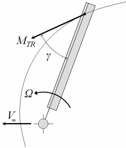
Figure 2.25. Trace Mach number geometry.
