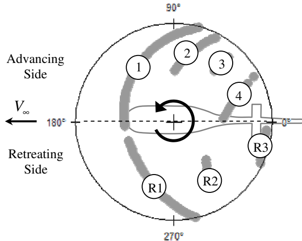
Figure 4.3. BVI Interaction Locations for a 2 bladed rotor at 60 knots ( \mu = 0.15 )
