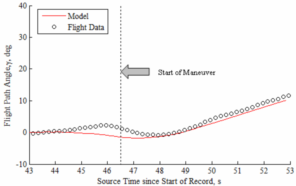
Figure 4.37. Slow pull-up flight path time history.
