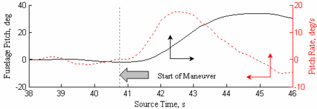
Figure 2.16. Body response during fast pull-up maneuver.
