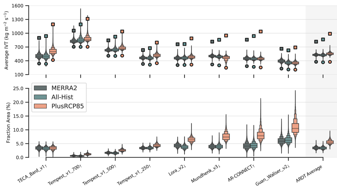
Figure 2. Boxplot of (top row) object-mean atmospheric river integrated vapor transport and (bottom row) fractional area for global atmospheric river detection tools (ARDTs) over the entire period (1979–2005, 2079–2099). The small boxes are mean object-maximum values over all time slices, small circles show mean object-minimum values over all time slices. Pink is the future climate, blue is the historical climate, and gray is MERRA-2. Global ARDTs are listed on the x-axis, and statistical boxes show the median (center line) with each outward level containing half the remaining data. Up (down) arrows next to ARDT names indicate restrictive (less restrictive) methods.
