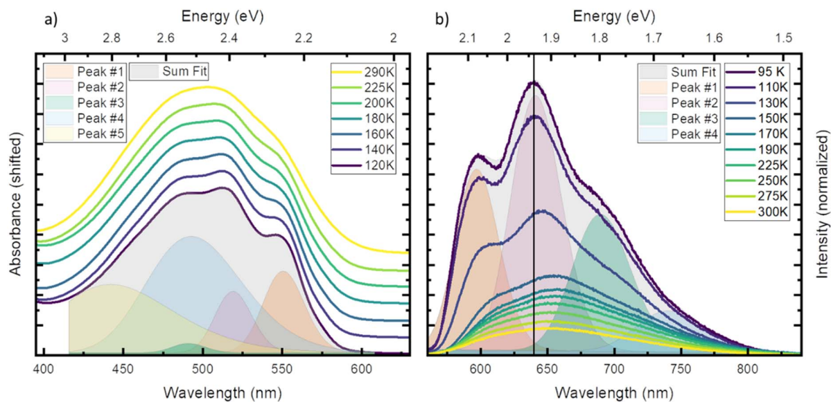
Fig. 1 Steady state absorption (a) and emission (b) in PrCN at different temperatures. (a) For comparability the spectra are normalized to the maximum and shifted vertically. (b) Emission spectra after excitation at 510 nm, drawn to scale. Both panels include the fit performed in energy scale of respective spectrum at the lowest measured temperature (grey area) and the individual Gaussian peaks (coloured areas).
