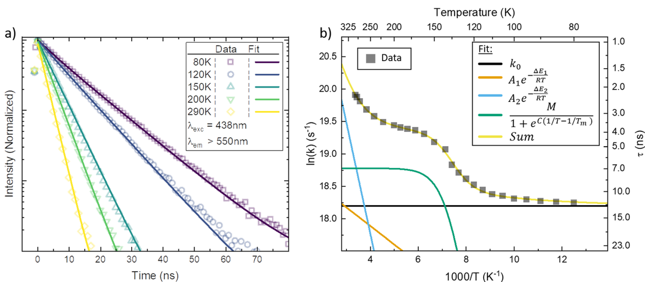
Fig. 3 (a) Temperature dependent luminescence decay measured by spectrally integrated time-correlated single photon counting (TCSPC) in PrCN. Data at selected temperatures are shown together with a double exponential fit to the data. (b) The major rate constant fitted to the TCSPC data (black squares) plotted as a function of inverse temperature together with the Arrhenius fit (yellow line) to the data. Additionally, the decomposition of the individual components in the Arrhenius fit is given (coloured lines).
