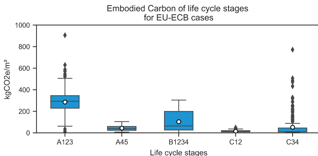
Figure 4. Embodied carbon per m 2 in different life cycle stages (A123, A45, B1234, C12, C34), based on EU-ECB baseline [11].
