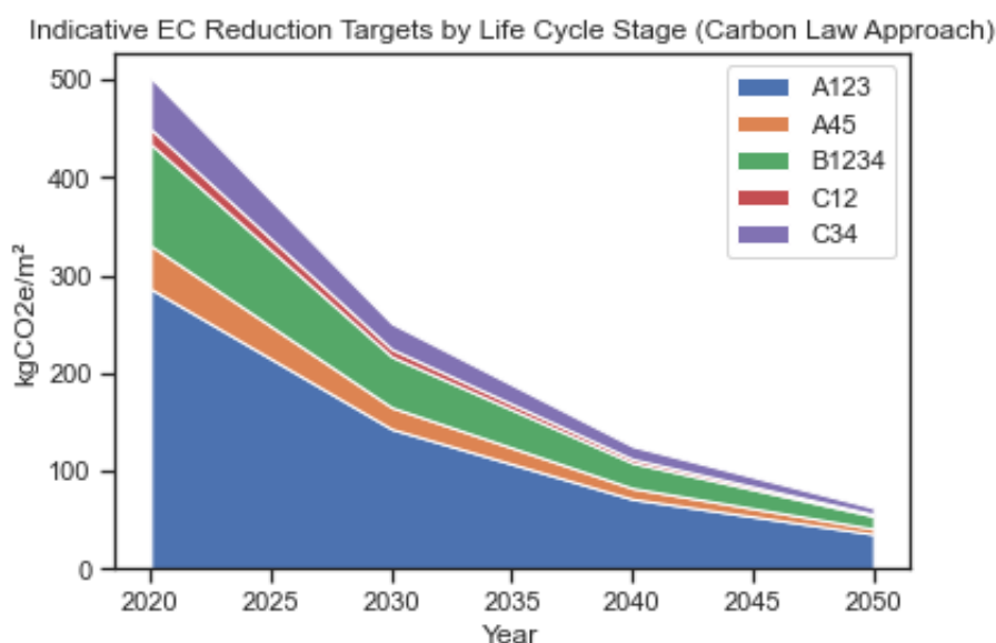
Figure 6. Indicative reduction targets for embodied carbon emission of both residential and non-residential buildings in different life cycle stages [ \text{kgCO}_2\text{e}/\text{m}^2 ], based on [11] and [12].
