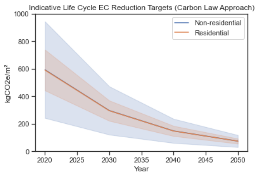
Figure 5. Indicative reduction targets for full life cycle embodied carbon emission [ \text{kgCO}_2\text{e/m}^2 ] of residential and non-residential buildings, respectively, based on [11] and [12].
