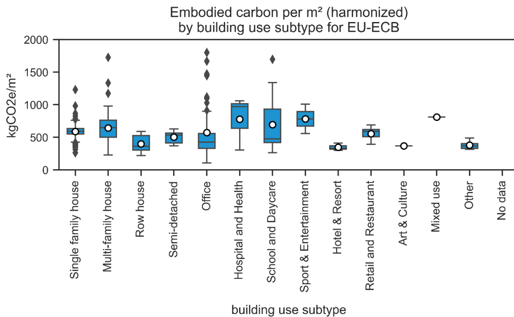
Figure 3. Life cycle embodied carbon per m 2 by building use subtype, based on EU-ECB baseline [11].
