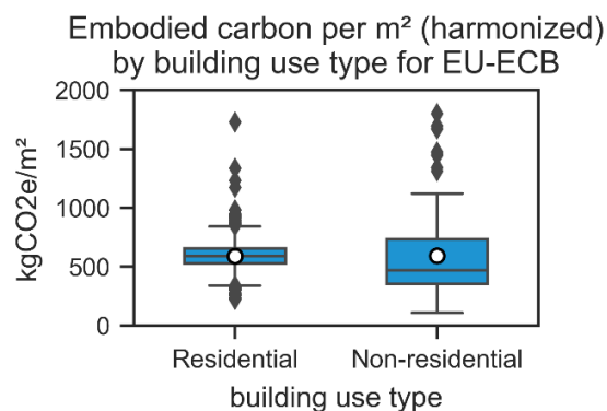
Figure 2. Life cycle embodied carbon per m 2 by building use type, based on EU-ECB baseline [11].
