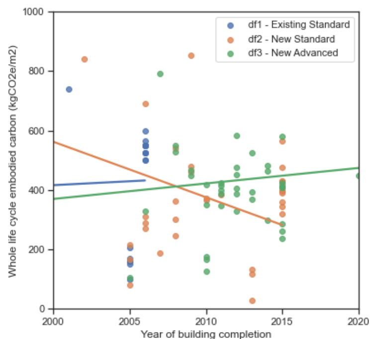
Figure 1. Historical development of embodied carbon per m 2 in IEA EBC Annex 72 dataset [3].
