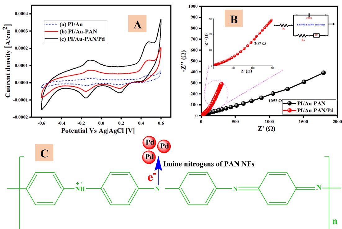
Fig. 4. (A) (a) PI/Au, (b) PI/Au-PAN NF, and (c) PI/Au-PAN/Pd in 0.5 M \text{H}_2\text{SO}_4 at a sweep rate of 100 \text{ mV s}^{-1} . (B) EIS spectra of PI/Au-PAN, and PI/Au-PAN/Pd flexible electrodes recorded in 0.1 M KCl containing 2 mM [\text{Fe}(\text{CN})_6]^{3-/4-} . Insets: Magnified portion and equivalent circuit of PI/Au-PAN/Pd electrode. (C) Mechanism of interaction between PAN NFs and Pd NRs.
