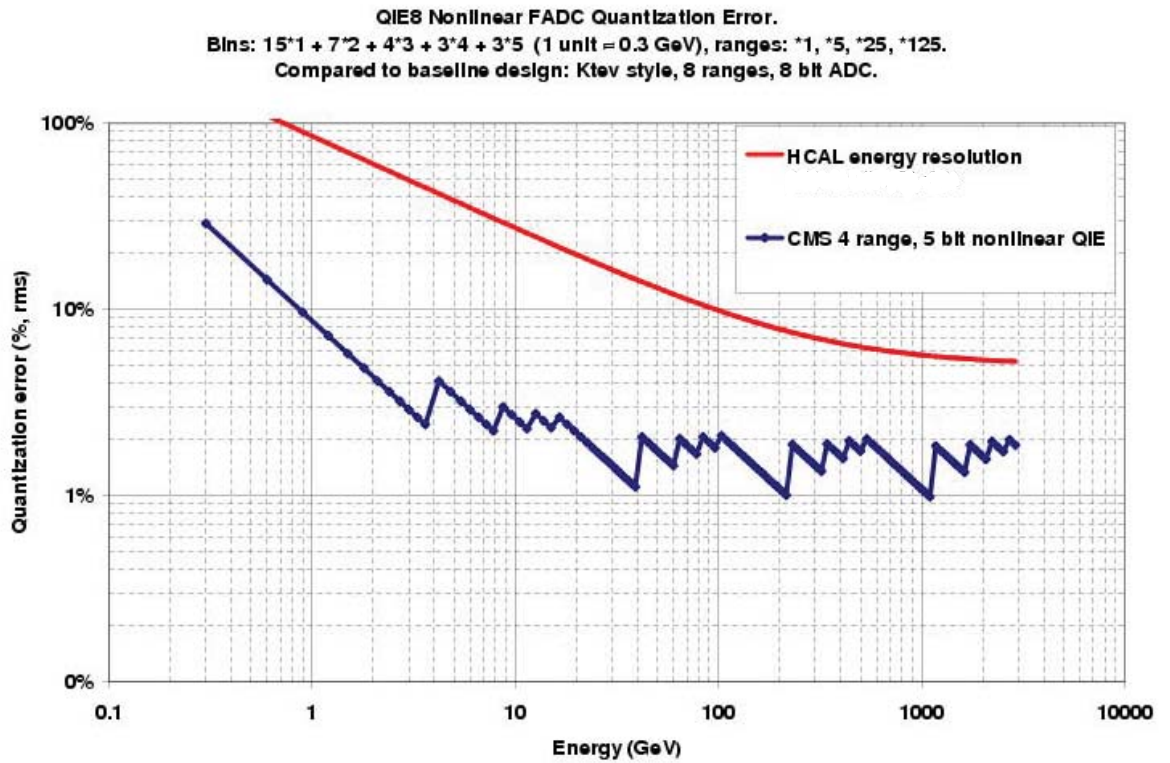
Figure 3.9: Quantization effects of the multi-linear scale of the HB analog-to-digital converters
