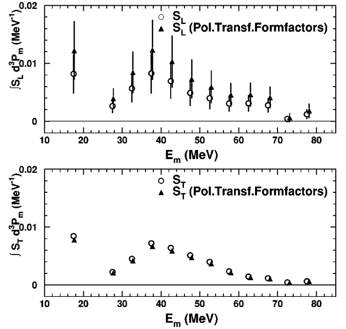
FIG. 20. Comparison of the carbon longitudinal (top panel) and transverse (bottom panel) spectral functions at Q^2=1.8 ( \text{GeV}/c ) ^2 , integrated over a p_m range 0 < p_m < 80 \text{MeV}/c , using the proton form factors obtained by the Rosenbluth separation [9,10] (open symbols) and the polarization transfer [11] methods (solid symbols). The lowest E_m point has been averaged over 10 < E_m < 25 \text{MeV} . The polarization transfer form factor points have been displaced slightly for clarity.
