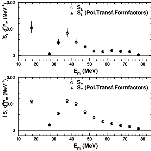
FIG. 19. Comparison of the carbon longitudinal (top panel) and transverse (bottom panel) spectral functions at Q^2=0.64 ( \text{GeV}/c ) ^2 , integrated over a p_m range 0 < p_m < 80 \text{MeV}/c , using the proton form factors obtained by the Rosenbluth separation [9,10] (open symbols) and the polarization transfer [11] methods (solid symbols). The lowest E_m point has been averaged over 10 < E_m < 25 \text{MeV} .
