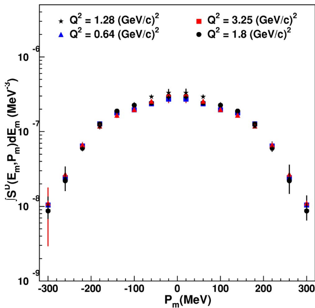
FIG. 7. (Color online) Momentum distributions for iron integrated over an E_m range 0 < E_m < 80 MeV. They have been normalized so that the integral of the measured spectral functions over |p_m| < 300 MeV/c is equal to the integral of the spectral function at Q^2 of 1.8 (GeV/c) 2 .
