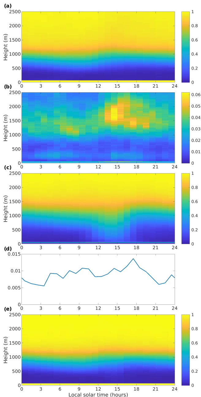
Figure 2. Fraction of Doppler lidar winds filtered at Granada by (a) the SNR filter, (b) the column-wise threshold filter, (c) the residual filter, (d) the rain filter, and (e) all filters combined. Note the change in colour scale for (b), since this filter is applied after the SNR filter. The rain filter is applied to the whole column. For panels (a)–(d), the fraction filtered refers to the winds at nominal temporal resolution (10–15 min) and for (e) to the 1 h averaged data.
