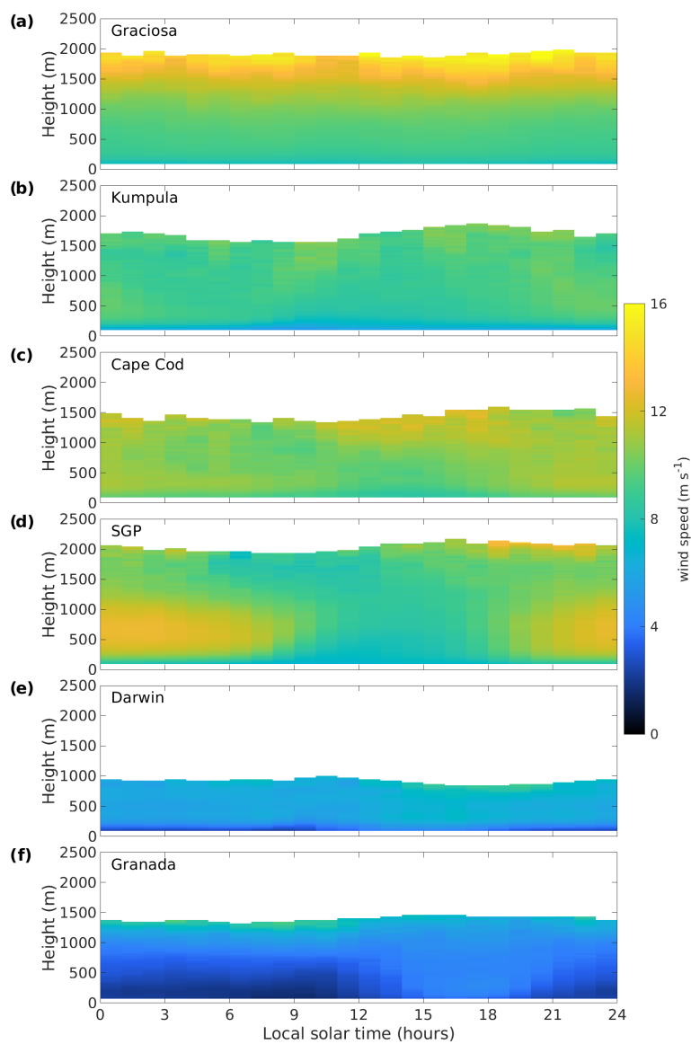
Figure A3. Diurnal composites of mean wind speed measured by the Doppler lidar at (a) Graciosa, (b) Kumpula, (c) Cape Cod, (d) SGP, (e) Darwin, and (f) Granada. Time refers to approximate local solar time.
