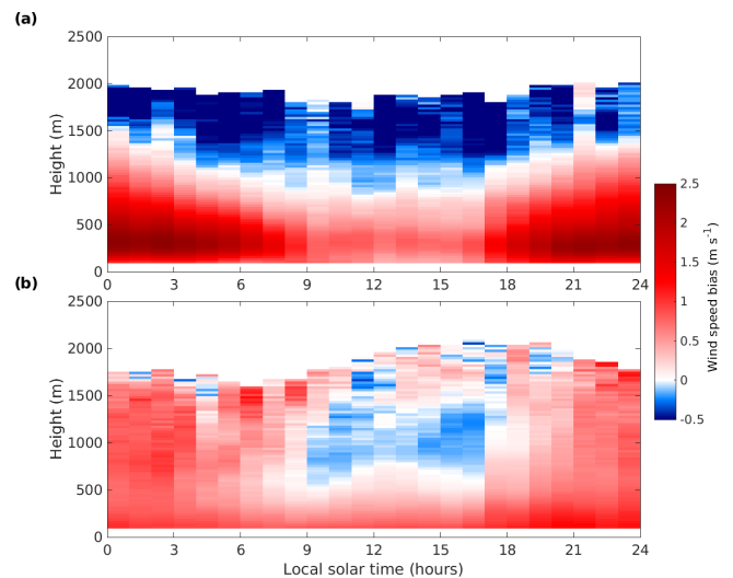
Figure 10. Composites of wind speed bias at SGP for when LLJ (a) is detected and (b) is not detected in the Doppler lidar data. Time refers to approximate local solar time.
