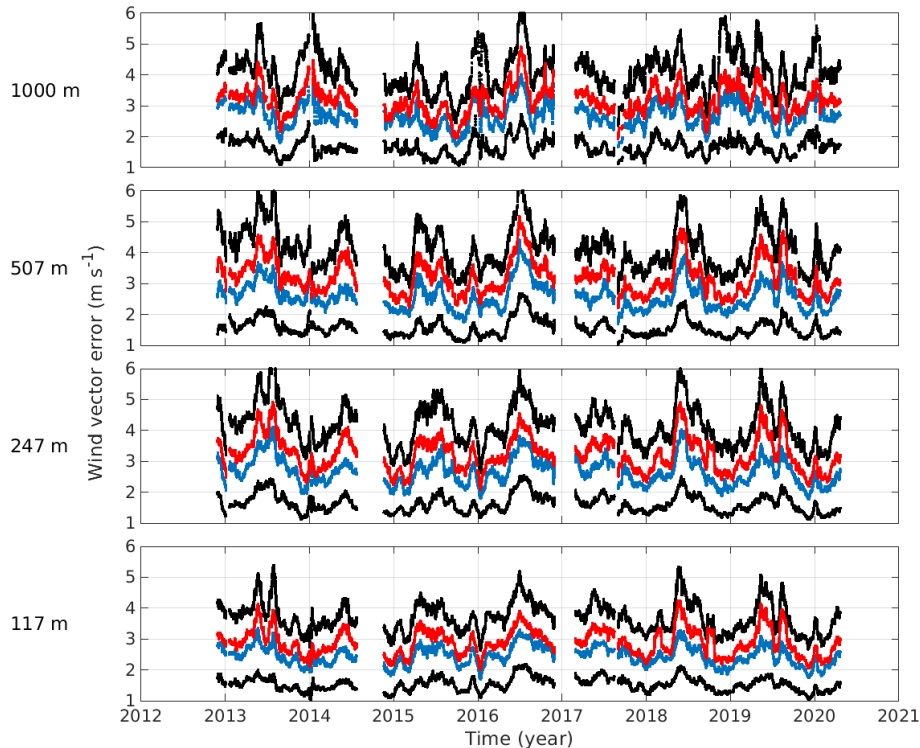
Figure 5. Time series of 30 d moving mean (red), median (blue), and 25th and 75th percentiles (black) of wind vector error over SGP at 117, 247, 507, and 1000 m a.g.l.
