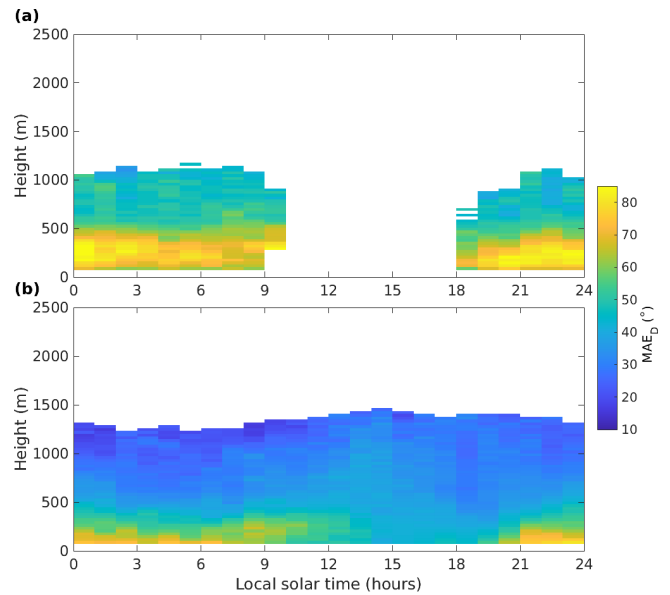
Figure 9. Diurnal composites of mean absolute wind direction error in Granada when a mountain breeze is (a) detected and (b) not detected in the Doppler lidar data. Time refers to approximate local solar time.
