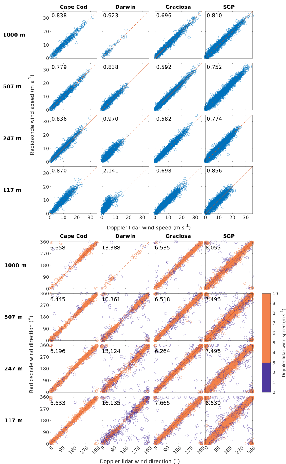
Figure 3. Scatter plots of Doppler lidar versus radiosonde wind speed and direction at four altitudes above ground level and at four locations. The mean absolute difference is also shown in each scatter plot. The wind direction is colour-coded in two classes with respect to the wind speed given by the Doppler lidar, denoting whether the wind speed was greater or less than 3 m s -1 .
