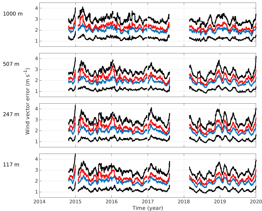
Figure A4. Time series of 30 d moving mean (red), median (blue), and 25th and 75th percentiles (black) of wind vector error over Graciosa at 117, 247, 507, and 1000 m a.g.l.
