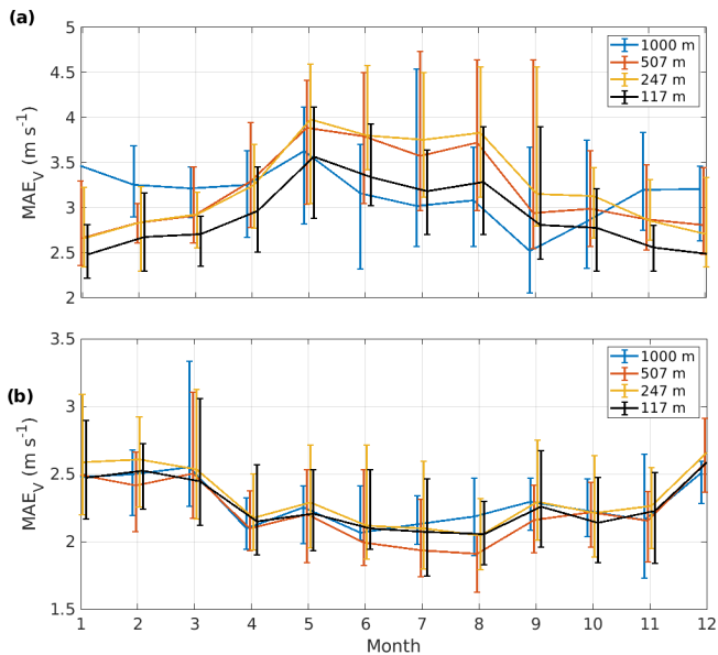
Figure 6. Monthly means of absolute wind vector error at (a) SGP and (b) Graciosa at 117, 247, 507, and 1000 m a.g.l. The bars show the maximum and minimum monthly average absolute wind vector error across all years.
