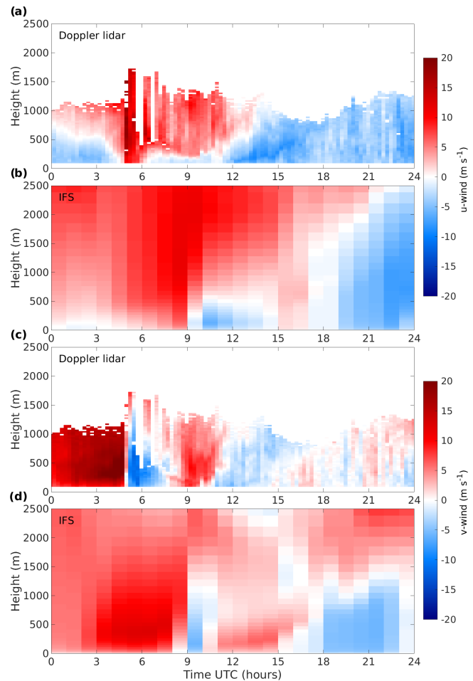
Figure 12. (a) Doppler lidar u wind, (b) IFS u wind, (c) Doppler lidar v wind, and (d) IFS v wind at SGP on 7 August 2013.
