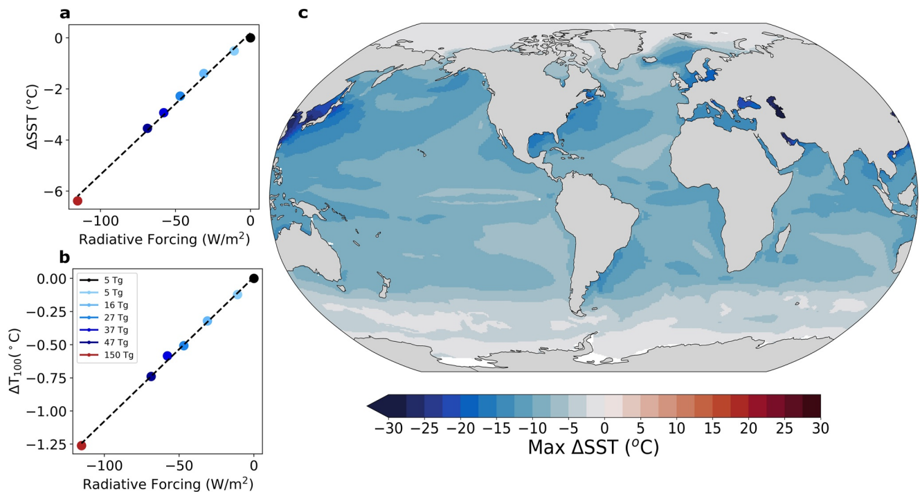
Figure 3. Global ocean temperature changes during and after nuclear war driven cooling. (a) Maximum annual global mean sea surface temperature anomaly ( \Delta SST) versus maximum radiative forcing anomaly for each war simulation. \Delta SST decreases linearly (dashed line), at a rate of 0.055^{\circ}\text{C W}^{-1}\text{m}^2 . (b) The global annual mean ocean temperature anomaly at 100 m ( \Delta T_{100} ) in 2034 (Year 15), indicating subsurface cooling in the new ocean state, also decreases linearly with radiation reduction at a rate of 0.011^{\circ}\text{C W}^{-1}\text{m}^2 (dashed). (c) Maximum monthly \Delta SST in the US-Russia (150 Tg) scenario at each model grid cell; ocean temperature anomalies are greatest in the Northern Hemisphere coastal regions and shallow seas. Anomalies are relative to the control mean.
