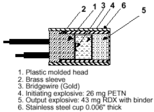
Figure 2. 2: RP-87 Explosive Train
