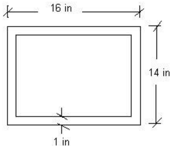
Figure 2.7: Frame Geometry
