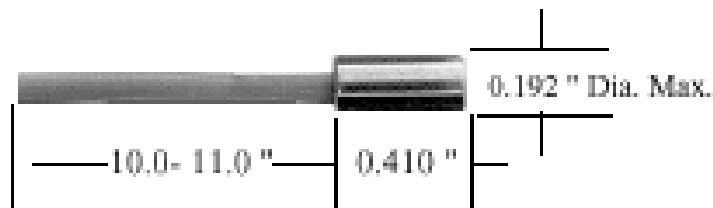
Figure 2. 1: RP-87 Dimensions
