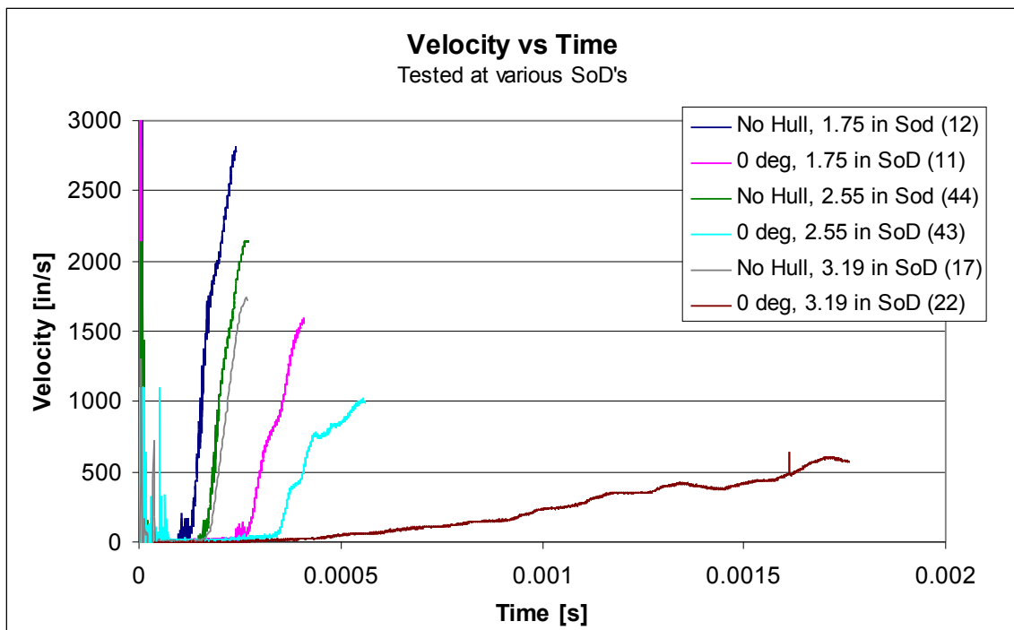
Figure 4.30: Velocity Profiles for tests conducted at various stand of distances
