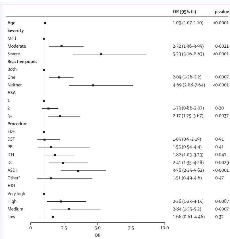
Figure 3: Factors associated with mortality in the mixed effects model
