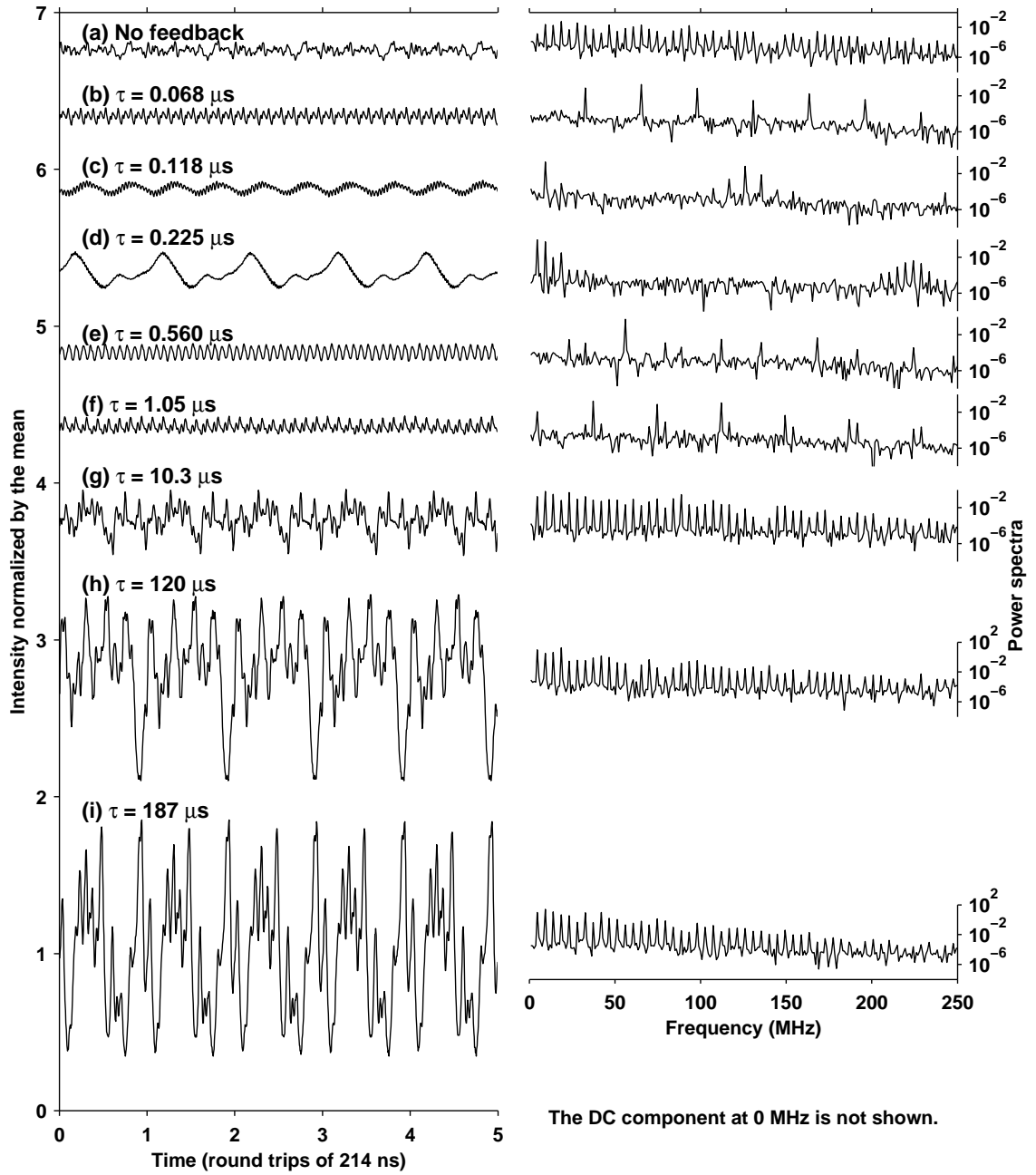
Figure 3.2: The left column shows laser output intensities over five round trips where the round trip time is 214 ns. Each time series is normalized by its mean, and the plots are offset for clarity. (a) is for the laser without feedback. (b)-(i) are for the laser with feedback with the time delay, \tau , given. The right hand column has power spectra of the five round trips shown for each time series. The DC component at 0 Hz has been omitted to better show the detail of the spectra.
