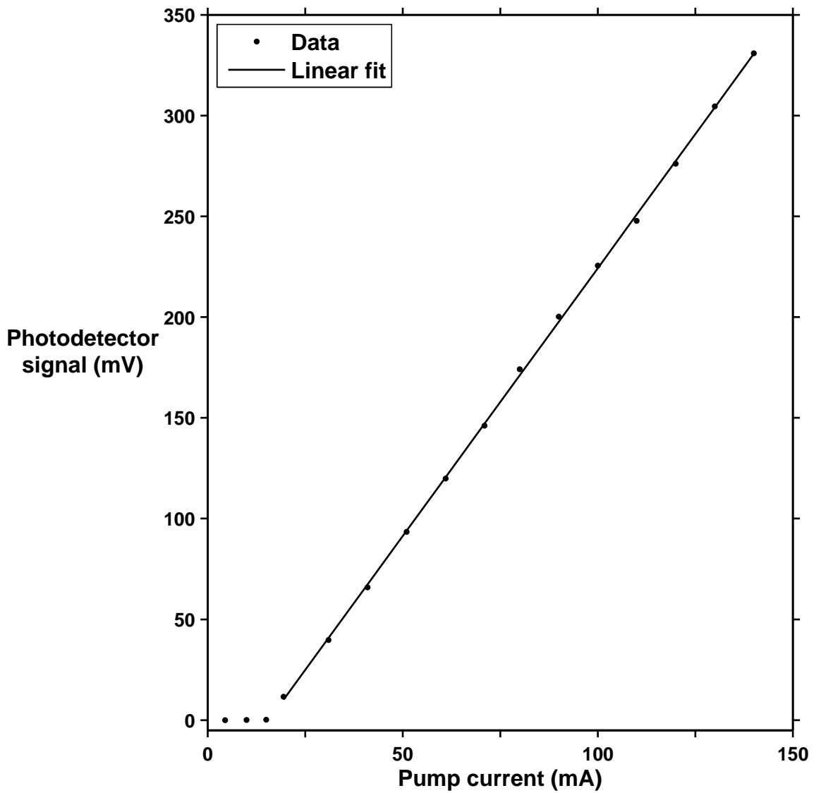
Figure 2.4: Laser power as a function of pump strength for the EDFRL. The power out is represented by the average photodetector signal as described in the text. The pump strength is represented by the pump current through the semiconductor laser used to pump the erbium ions.
