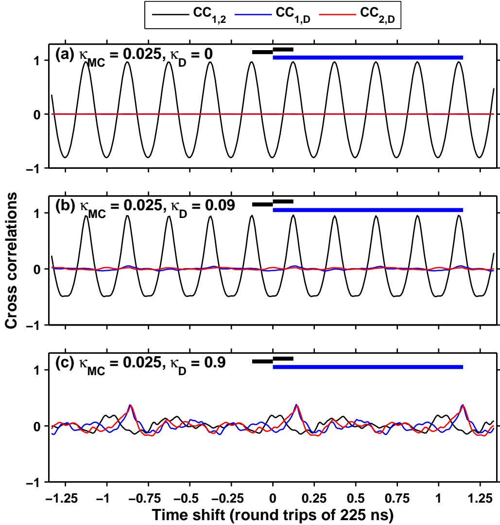
Figure 5.7: Cross correlations for unidirectional driving of mutually coupled response lasers pumped at 1.4I_{th} . (a) Mutual coupling between the response lasers only. (b) Low level of drive coupling. (c) High level of drive coupling. For all plots of CC_{x,y} the left(right) side of the plots correspond to a shift as if x(y) were leading. The blue bars indicate the 258 ns time lag for a signal to travel from the drive through the transmission line and the response laser and be measured as compared to a signal measured directly from the drive. The black bars indicate a symmetric shift of \pm 28 ns where CC_{1,2} should peak if lag synchrony between the response lasers is present.
