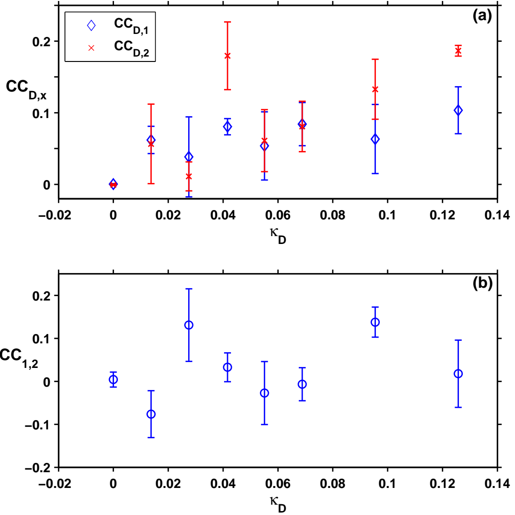
Figure 5.3: Cross correlations at specific shifts for unidirectional driving of uncoupled response lasers pumped at 4I_{th} . (a) Cross correlations between the drive and laser 1 (blue \diamond ) and the drive and laser 2 (red \times ) where the drive leads by s = 256 ns. (b) Cross correlation of laser 1 and 2 with s = 0 ns. The \kappa_D values are averages of the values for the two transmission lines.
