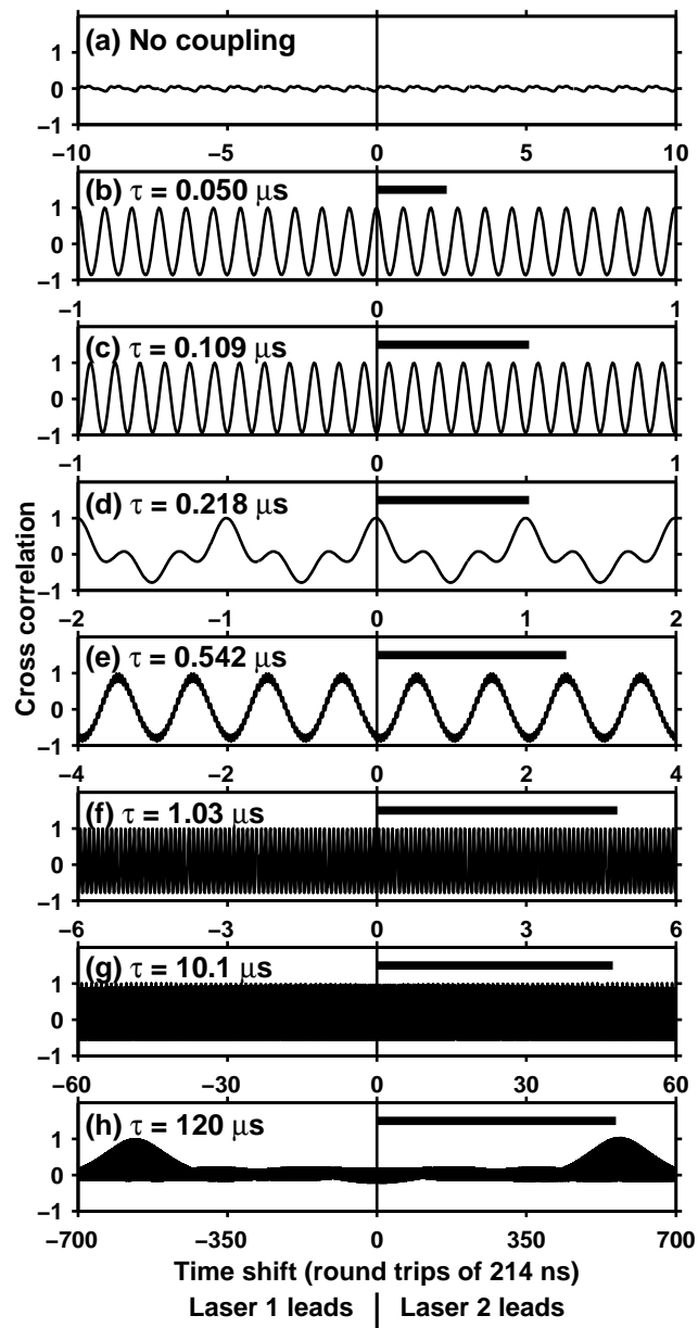
Figure 4.5: Cross correlations of the entire 1 ms intensity time series corresponding to the time series pairs shown in Fig 4.2. Plot (a) is for the uncoupled lasers. The rest of the plots are for the mutually coupled lasers with the time delay, \tau , given. The thick black bars show the delay time graphically. Note that the horizontal scale of each plot changes. Negative(positive) time shifts correspond to laser 1(2) leading. Due to the symmetry a definite leader cannot be determined with these plots.
