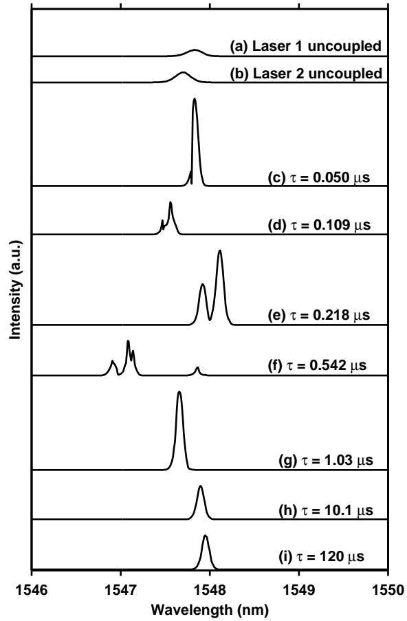
Figure 4.14: Optical spectra of the lasers. (a) and (b) are for the uncoupled lasers. (c)-(h) are the sum of the light from both lasers coupled with a delay, \tau , as listed.
