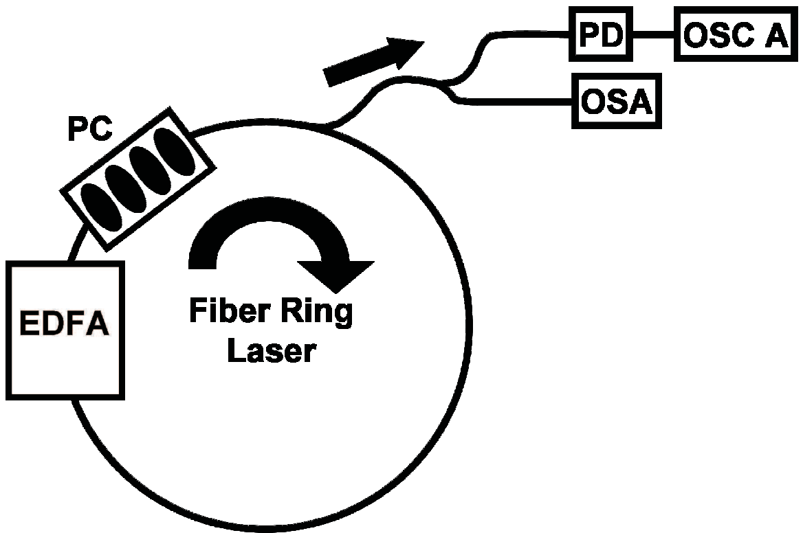
Figure 2.3: Experimental setup for the EDFRL. The arrows show the direction of light propagation through the ring. EDFA, erbium-doped fiber amplifier; PC, polarization controller consisting of a sequence of linear polarizer, quarter wave plate, half wave plate, and quarter wave plate; PD, photodetector; OSC A, oscilloscope used to measure the laser intensity dynamics; OSA, optical spectrum analyzer.
