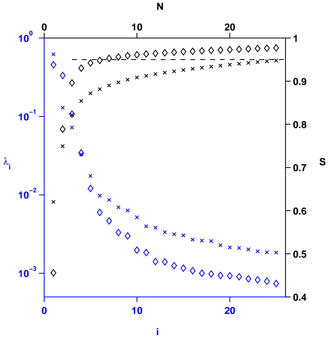
Figure 4.13: KL eigenvalue spectra and cumulative sum of the eigenvalues for laser 1 ( \diamond ) and laser 2 ( \times ) uncoupled. The first 25 normalized eigenvalues are plotted on the left axis in blue and the cumulative sum of the eigenvalues is plotted in black on the right axis. The dotted line shows the the cut off S = 0.95 .
