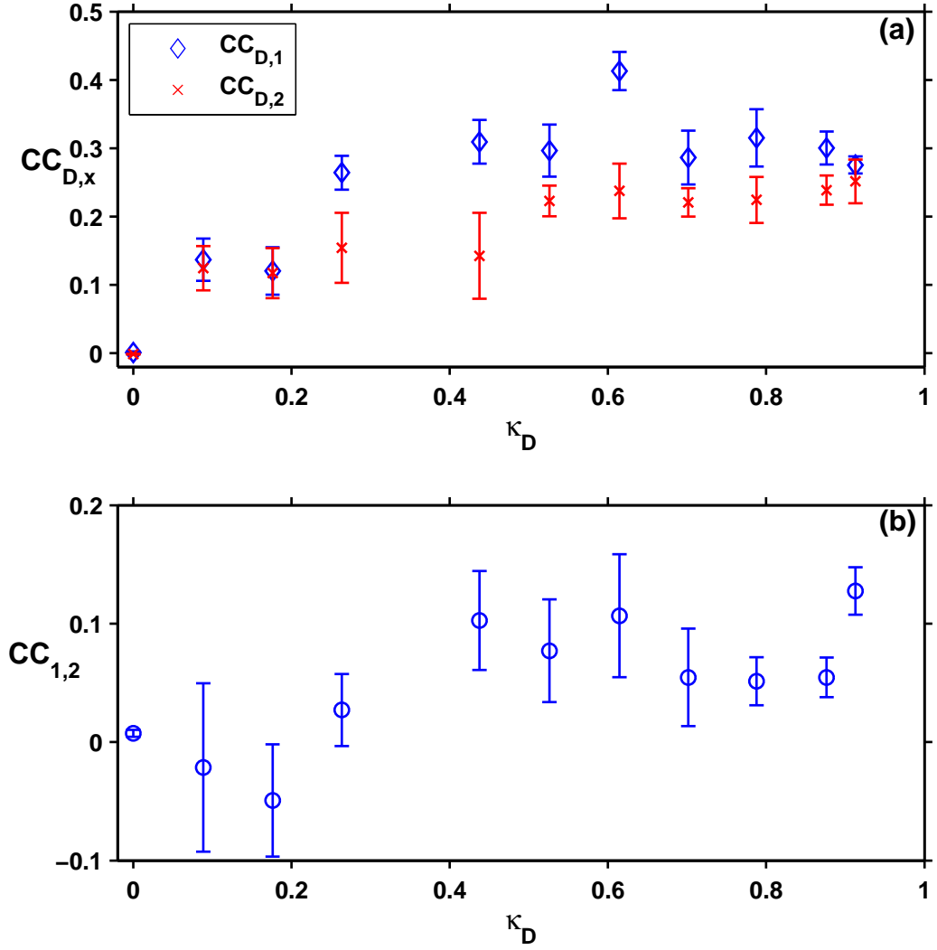
Figure 5.5: Cross correlations at specific shifts for unidirectional driving of uncoupled response lasers pumped at 1.4I_{th} . (a) Cross correlations between the drive and laser 1 (blue \diamond ) and the drive and laser 2 (red \times ) where the drive leads by s = 258 ns. (b) Cross correlation of laser 1 and 2 with s = 0 ns. The \kappa_D values are averages of the values for the two transmission lines.
