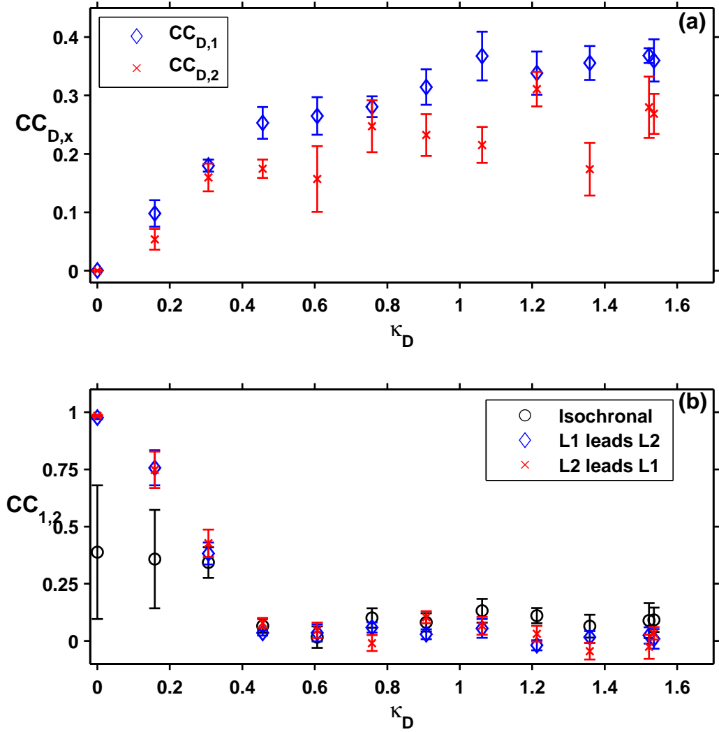
Figure 5.10: Cross correlations at specific shifts for unidirectional driving of mutually coupled response lasers pumped at 1.2I_{th} . (a) Cross correlations at specific shifts between the drive and laser 1 (blue \diamond ) and the drive and laser 2 (red \times ) where the drive leads by s = 256 ns. (b) Cross correlations of laser 1 and 2 with no shift ( s = 0 ns, \circ ), shifted so laser 1 leads ( s = -28 ns, blue \diamond ), and shifted so laser 2 leads ( s = 28 ns, red \times ). The \kappa_D values are averages of the values for the two transmission lines.
