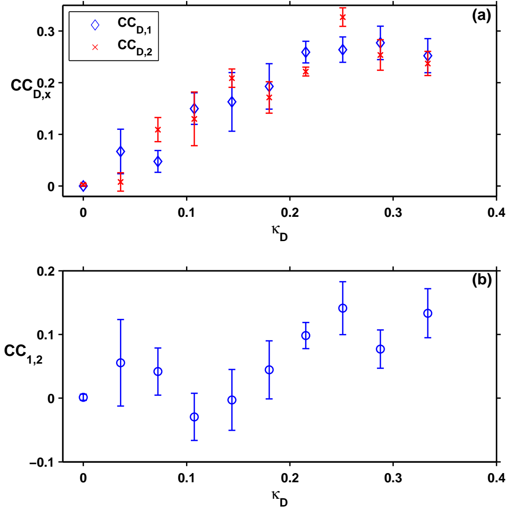
Figure 5.4: Cross correlations at specific shifts for unidirectional driving of uncoupled response lasers pumped at 2I_{th} . (a) Cross correlations between the drive and laser 1 (blue \diamond ) and the drive and laser 2 (red \times ) where the drive leads by s = 256 ns. (b) Cross correlation of laser 1 and 2 with s = 0 ns. The \kappa_D values are averages of the values for the two transmission lines.
