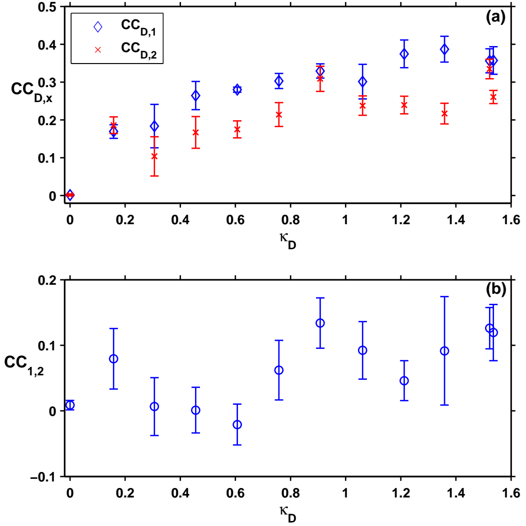
Figure 5.6: Cross correlations at specific shifts for unidirectional driving of uncoupled response lasers pumped at 1.2I_{th} . (a) Cross correlations between the drive and laser 1 (blue \diamond ) and the drive and laser 2 (red \times ) where the drive leads by s = 258 ns. (b) Cross correlation of laser 1 and 2 with s = 0 ns. The \kappa_D values are averages of the values for the two transmission lines.
