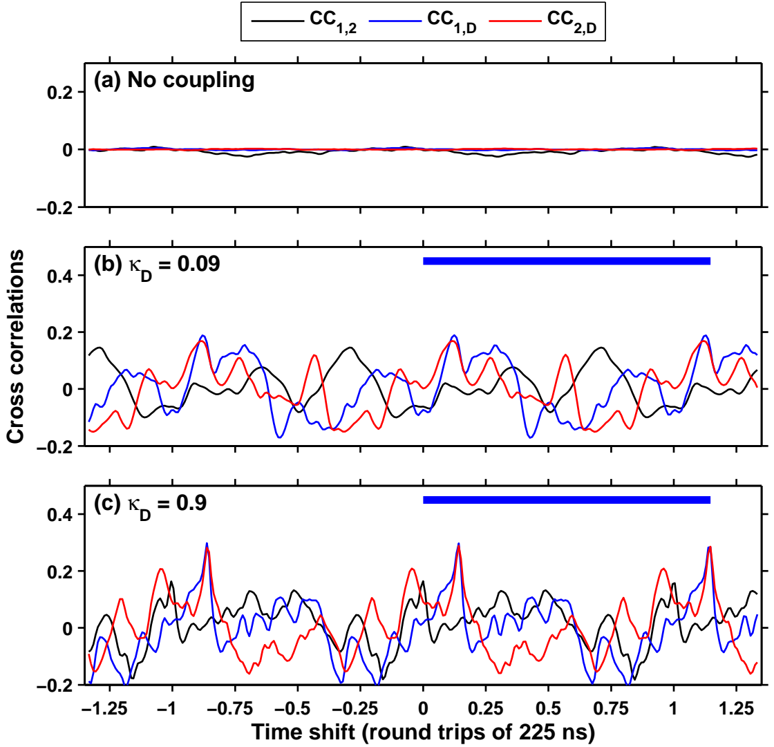
Figure 5.2: Cross correlations for unidirectional driving of uncoupled response lasers pumped at 1.4I_{th} . (a) No coupling between any of the lasers. (b) Low level of drive coupling. (c) High level of drive coupling. For all plots of CC_{x,y} the left(right) side of the plots correspond to a shift as if x(y) were leading. The blue bars in plots (b) and (c) indicate the 258 ns time lag for a signal to travel from the drive through the transmission line and the response laser and be measured as compared to a signal measured directly from the drive.
