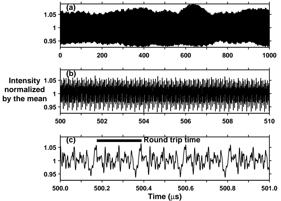
Figure 2.5: Intensity time series for the EDFRL. (a) Entire 1 ms time series normalized by the mean. (b) Ten \mu\text{s} portion of the time series in (a). (c) One \mu\text{s} portion of the time series in (b). The round trip pattern repetition is visible in this plot.
