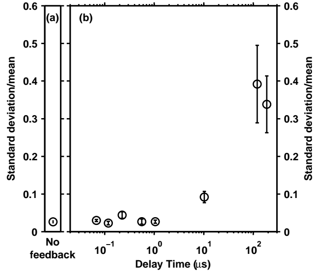
Figure 3.3: (a) Ratio of standard deviation to the mean for the laser without feedback. (b) Ratio of standard deviation to the mean for the laser with feedback of different delays. The error bars in both plots are the statistical standard error based on a sample set of five 1 ms long time series.
