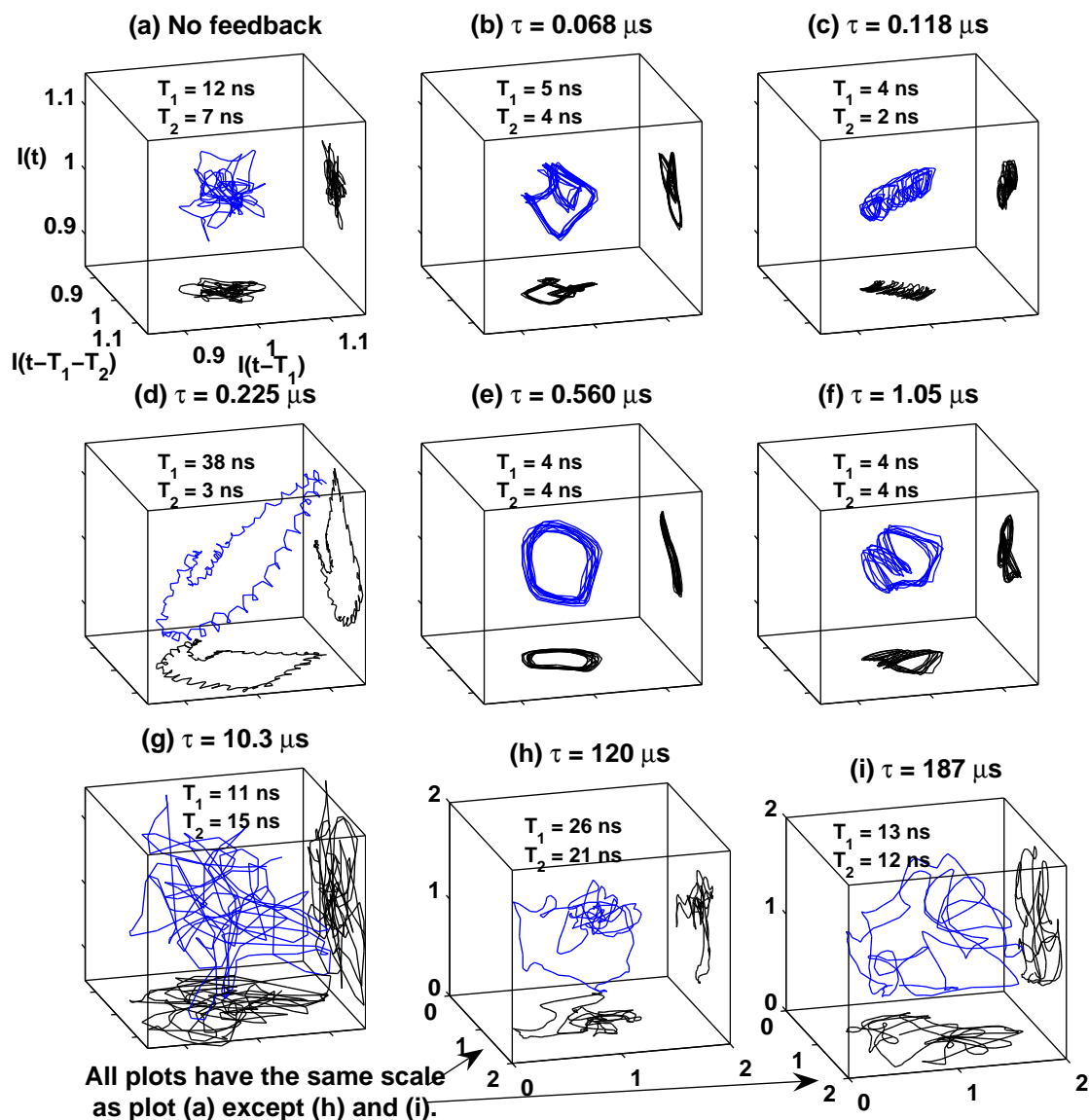
Figure 3.4: Time delay embeddings of the first round trip shown in Fig. 3.2. Plot (a) is for the laser without feedback. The rest of the plots are for the laser with feedback with the time delay, \tau , given. The embedding delays, T_1 and T_2 , are also given. The blue curve is the 3-D trajectory, and the black curves are 2-D projections onto the bottom and right sides of the plots. The data points are 1 ns apart. Plots (a) through (g) have the same scale. Plots (h) and (i) have a larger scale due to the larger fluctuations in these time series. The plots are centered about 1 because each time series was normalized to its mean.
