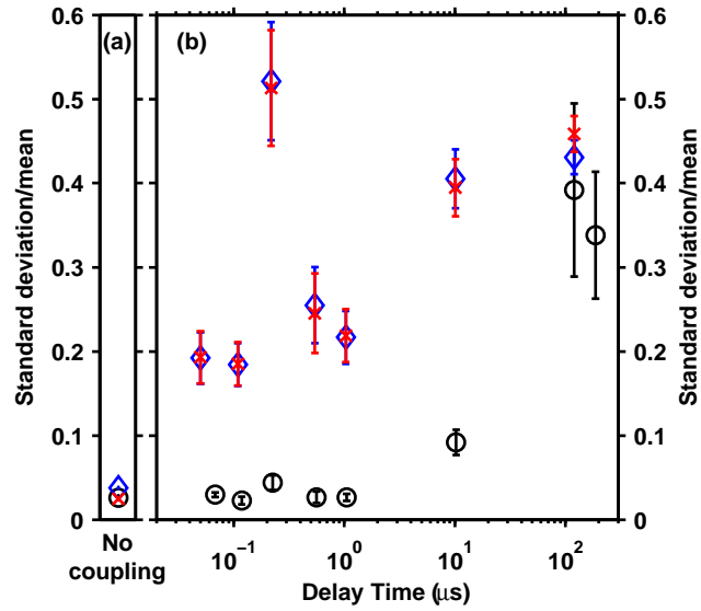
Figure 4.3: (a) Ratio of standard deviation to the mean for a single laser without feedback ( \circ ) and laser 1 (blue \diamond ) and laser 2 (red \times ) when uncoupled. (b) Ratio of standard deviation to the mean for single laser with feedback ( \circ ) and laser 1 (blue \diamond ) coupled to laser 2 (red \times ) with different delays. The error bars in both plots are the statistical standard error based on a sample set of ten for the coupled lasers and five for the single laser. The single laser data ( \circ ) are reprinted from Fig. 3.3 for comparison.
