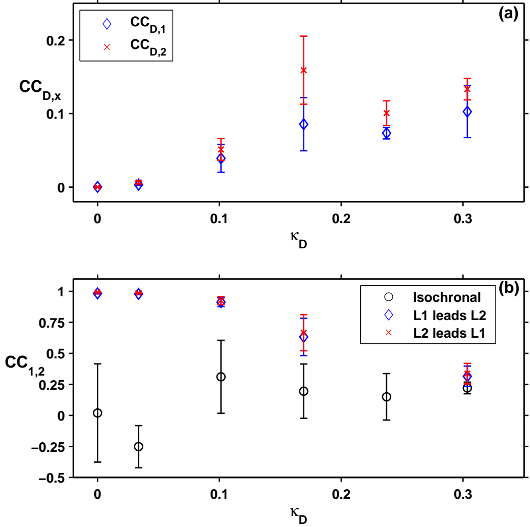
Figure 5.8: Cross correlations at specific shifts for unidirectional driving of mutually coupled response lasers pumped at 2I_{th} . (a) Cross correlations at specific shifts between the drive and laser 1 (blue \diamond ) and the drive and laser 2 (red \times ) where the drive leads by s = 256 ns. (b) Cross correlations of laser 1 and 2 with no shift ( s = 0 ns, \circ ), shifted so laser 1 leads ( s = -28 ns, blue \diamond ), and shifted so laser 2 leads ( s = 28 ns, red \times ). The \kappa_D values are averages of the values for the two transmission lines.
