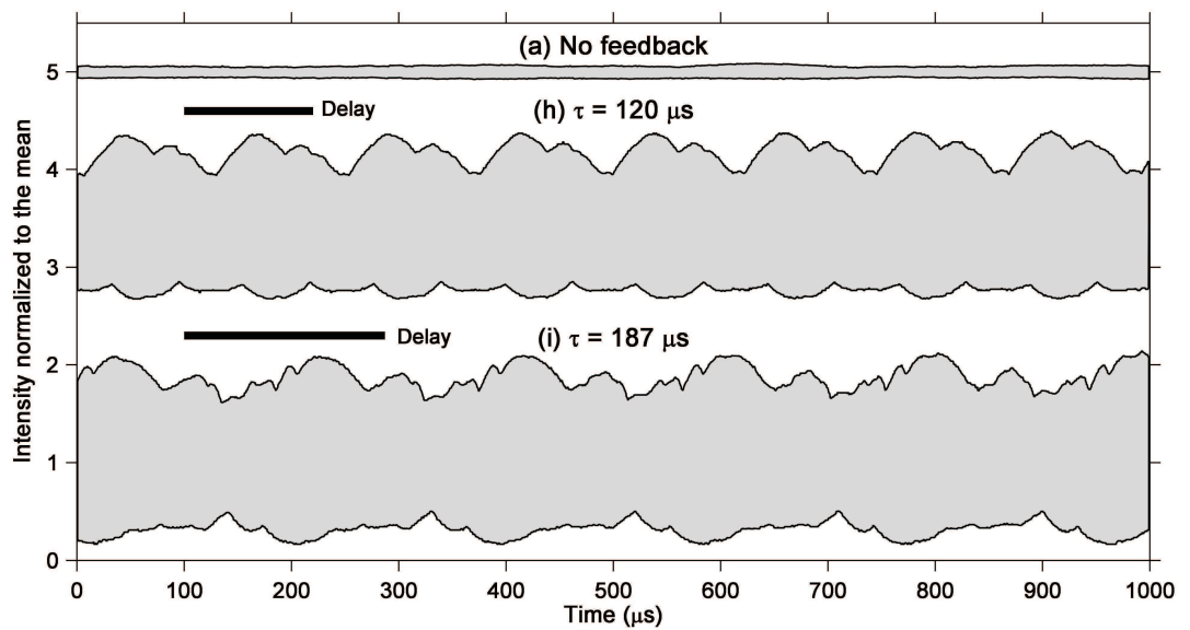
Figure 3.6: Envelope of the full 1 ms time series of the intensity dynamics for a laser with (a) no feedback and (h)-(i) feedback with the time delay, \tau , listed. The labeling corresponds to the plots in previous figures. (a) and (h) are offset for clarity. The bars on plots (h) and (i) visually show the length of \tau for each plot.
