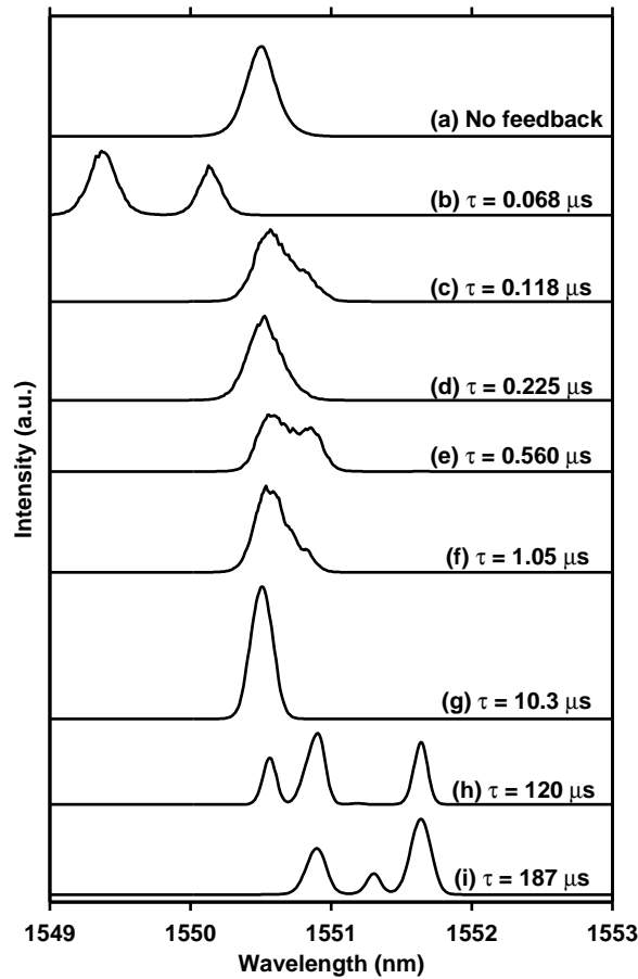
Figure 3.13: Optical spectra of the laser. (a) is for the laser without feedback. (b)-(i) are for a laser with feedback with a delay, \tau , as listed.
