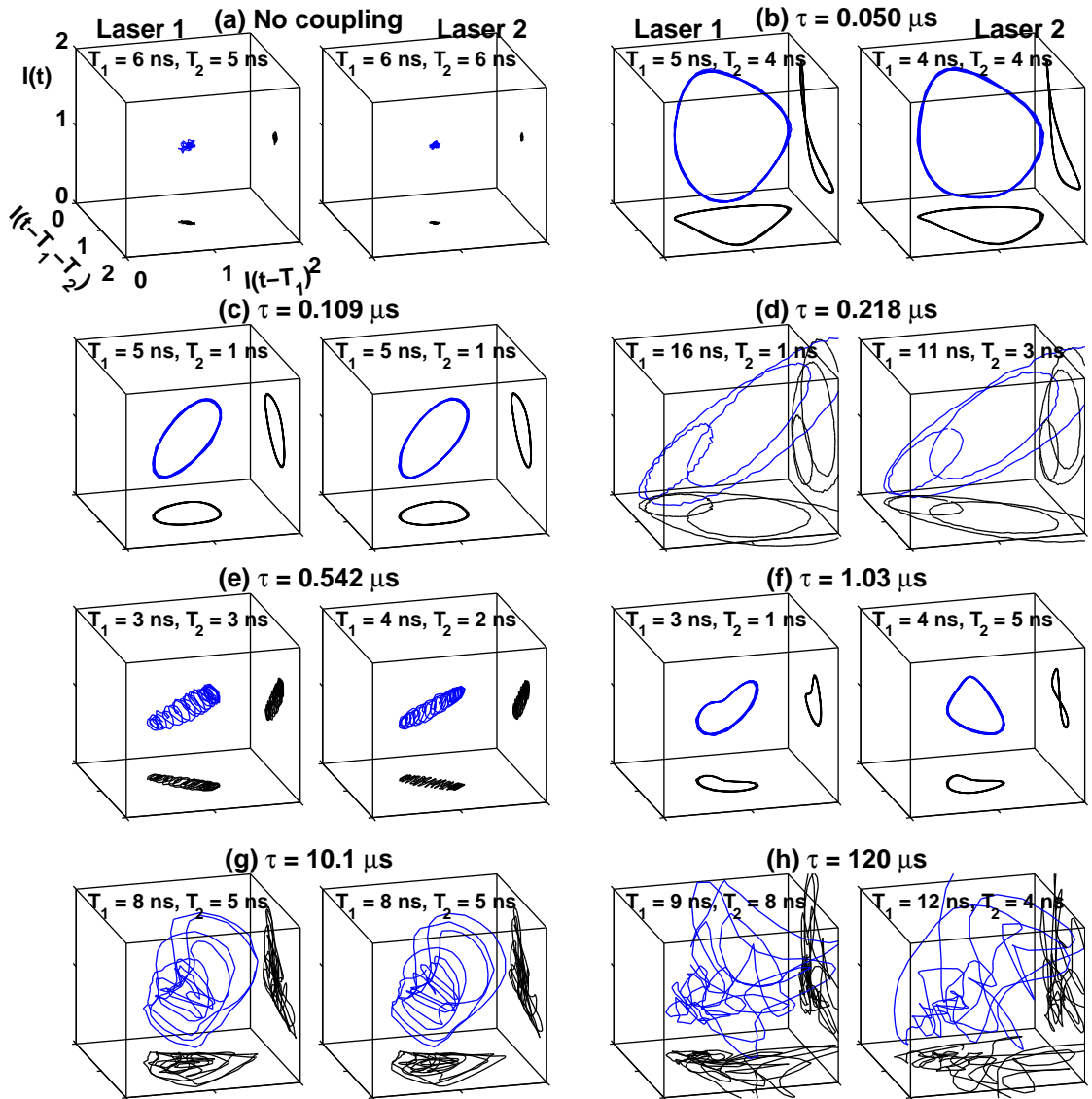
Figure 4.4: Time delay embeddings of the first round trip shown in Fig 4.2. Laser 1 is shown in the left box, and laser 2 is shown in the right box for each pair. Plot (a) is for the uncoupled lasers. The rest of the plots are for the mutually coupled lasers with the time delay, \tau , given. The embedding delays, T_1 and T_2 , are also given. The blue curve is the 3-D trajectory, and the black curves are 2-D projections onto the bottom and right sides of the plots. The data points are 1 ns apart. All plots have the same scale and are centered about 1 because each time series was normalized by its mean.
