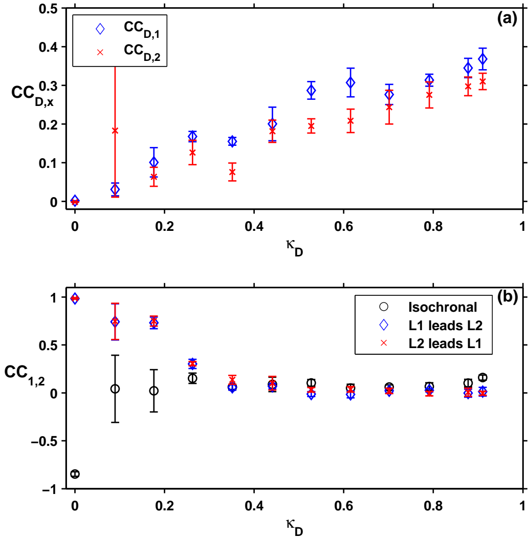
Figure 5.9: Cross correlations at specific shifts for unidirectional driving of mutually coupled response lasers pumped at 1.4I_{th} . (a) Cross correlations at specific shifts between the drive and laser 1 (blue \diamond ) and the drive and laser 2 (red \times ) where the drive leads by s = 258 ns. (b) Cross correlations of laser 1 and 2 with no shift ( s = 0 ns, \circ ), shifted so laser 1 leads ( s = -28 ns, blue \diamond ), and shifted so laser 2 leads ( s = 28 ns, red \times ). The \kappa_D values are averages of the values for the two transmission lines.
