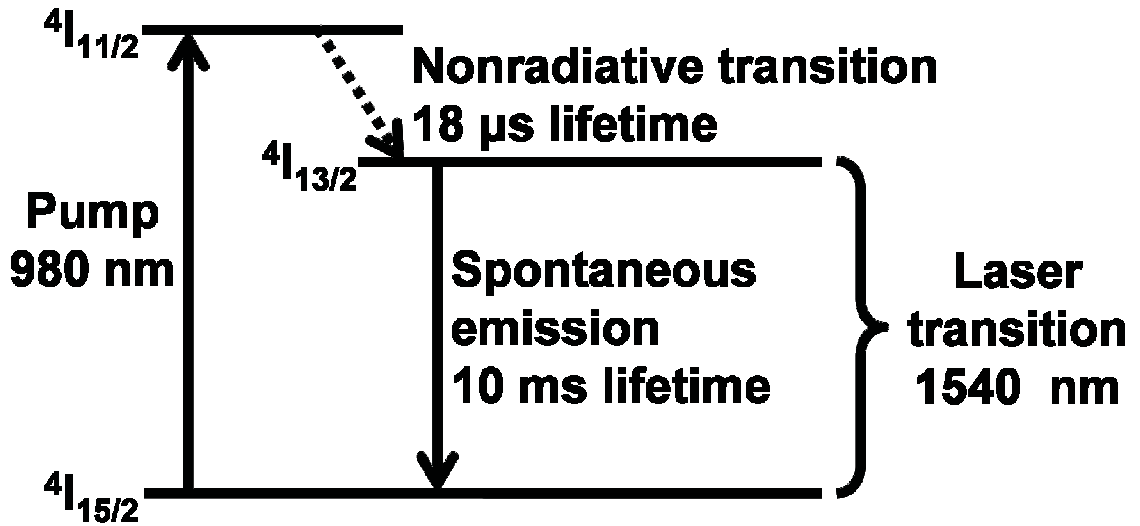
Figure 2.1: Erbium ion energy levels used by the laser. Erbium ions are pumped to the 4I_{11/2} level where they quickly decay nonradiatively to the metastable 4I_{13/2} level. Laser light comes from stimulated emission from the metastable level to the ground level transition. Data in the figure is from [69].
