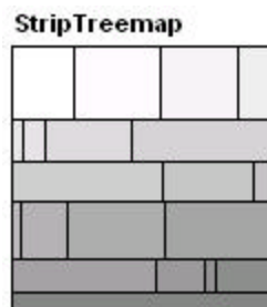
Figure 6: Strip treemap algorithm applied to 20 rectangles.
