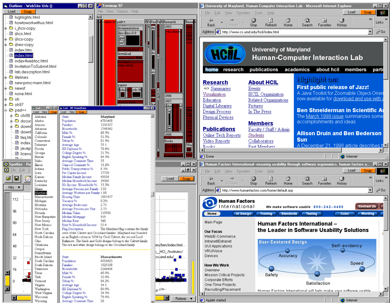
Figure 4: This visualization environment for exploring website log data was quickly constructed using Snap. The outliner, Treemap, and web browser at the top start the Snap tool, and browser for the HCIL website. The scatter plot and browser at the bottom display pages that refer readers to the site. This example reveals that Human Factors International referred 110 readers to the HCIL home page that month.
