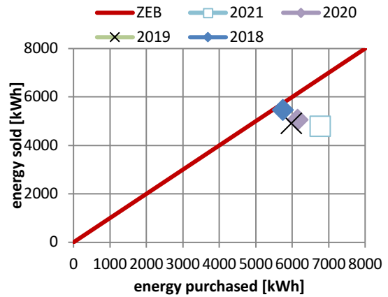
Fig. 3 - Annual electricity purchased and sold (2018-2021).
