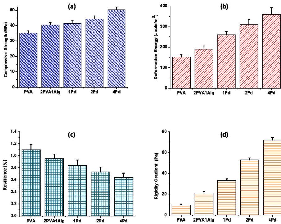
Figure (5). Physico-mechanical properties of the prepared scaffolds represented by (a) compressive strength; (b) deformation energy; (c) matrix resilience and (d) rigidity Gradient.
