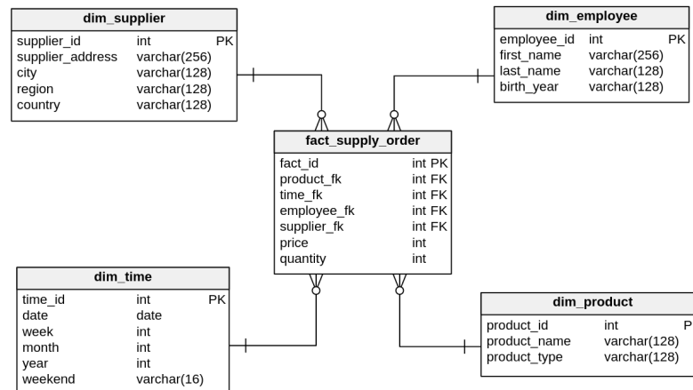
Figure 14: Star schema example
