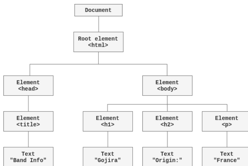
Figure 8: Webpage DOM example.
