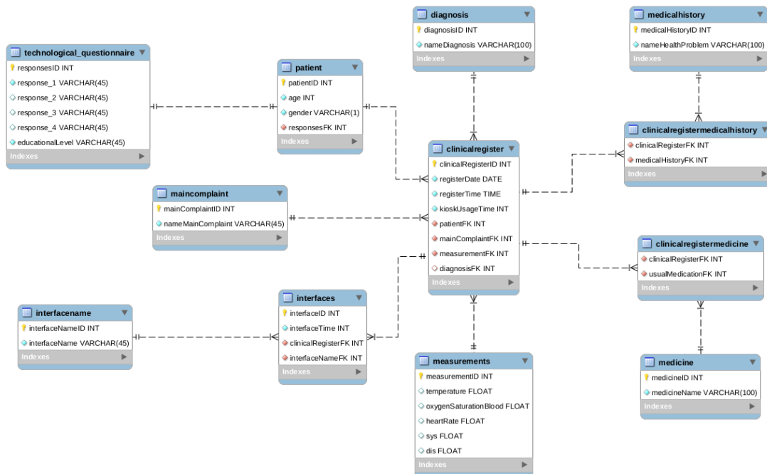
Figure 63: Staging Area
