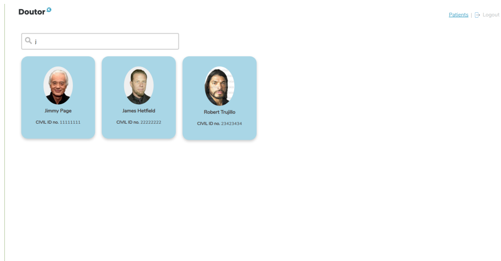
Figure 59: SearchInput component
