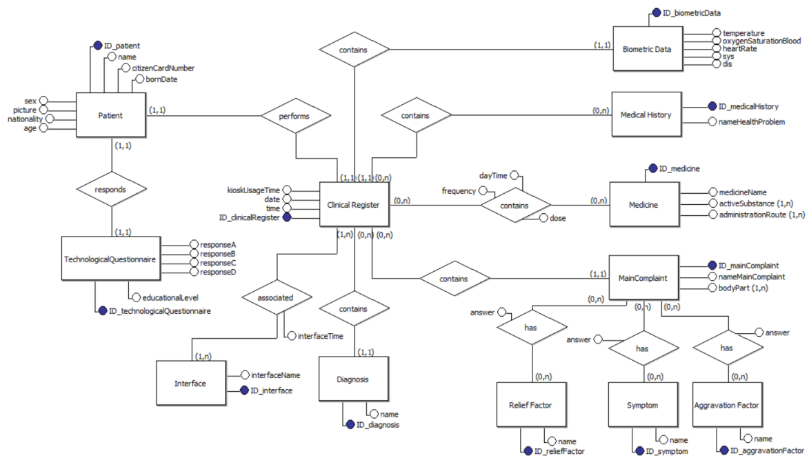
Figure 20: Conceptual model
