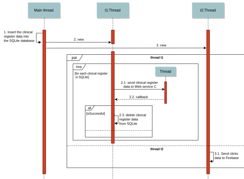
Figure 43: Sequence diagram illustrating the data storage process of the second version of the android application
