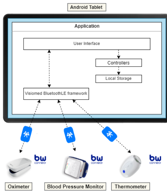
Figure 31: First version architecture
