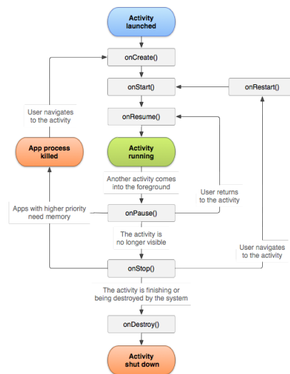
Figure 5: Activity lifecycle, adopted from [20]
