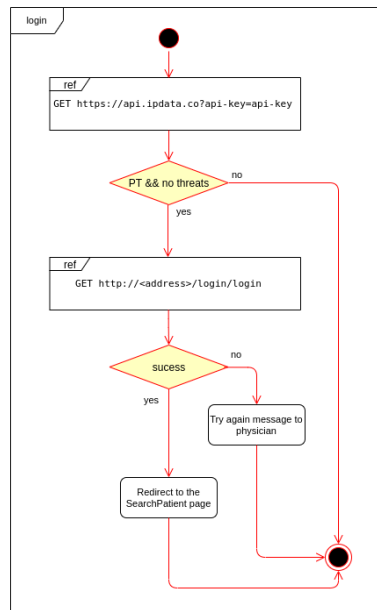
Figure 56: Diagram of activities illustrating the Web application authentication process
