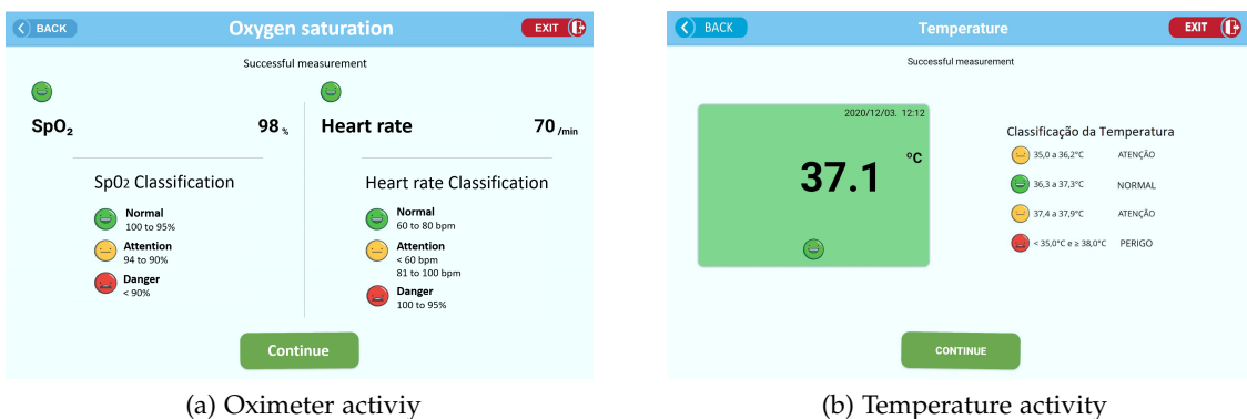
Figure 40: First version, oximeter and temperature interfaces
