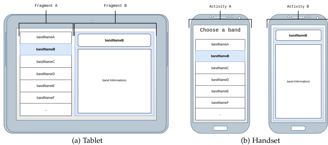
Figure 7: Example of the use of activities and fragments.
