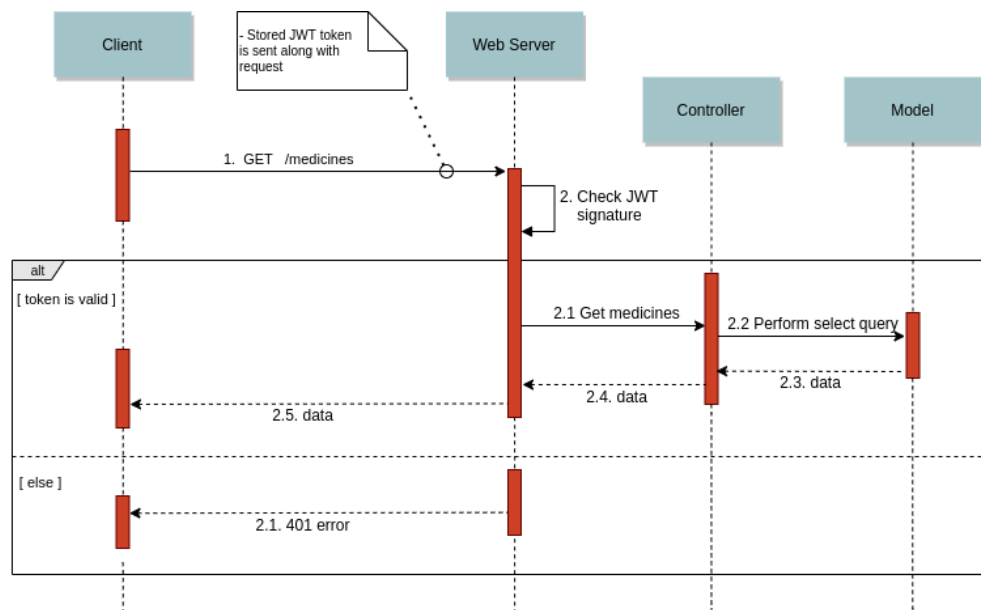
Figure 30: Sequence diagram showing the interactions between the client and the Web service performing a request
