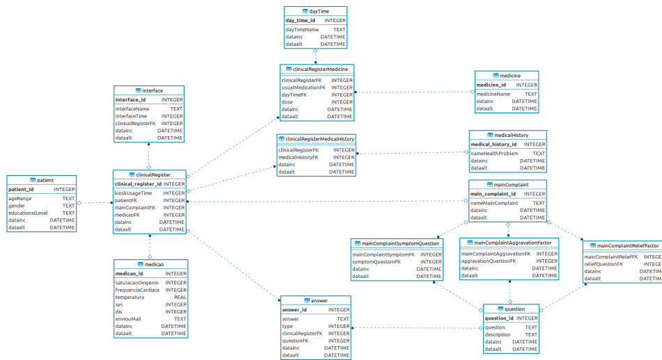
Figure 34: SQLite database of the first Android application prototype
