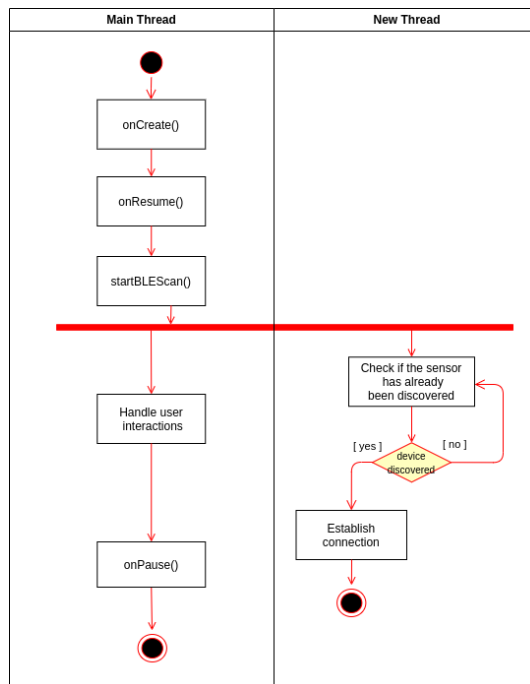
Figure 33: Activity diagram showing the search process and connection of each sensor
