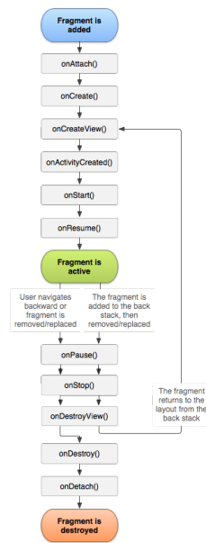
Figure 6: Fragment lifecycle, adopted from [21]
