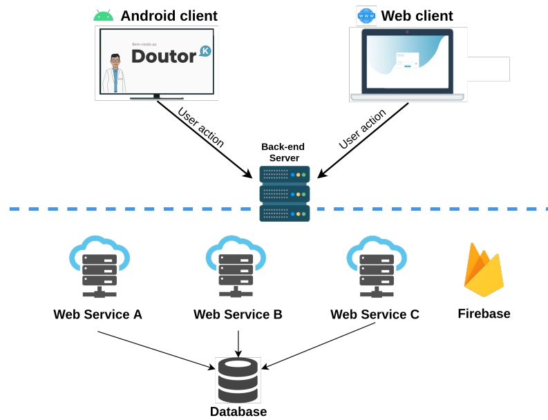
Figure 17: System architecture
