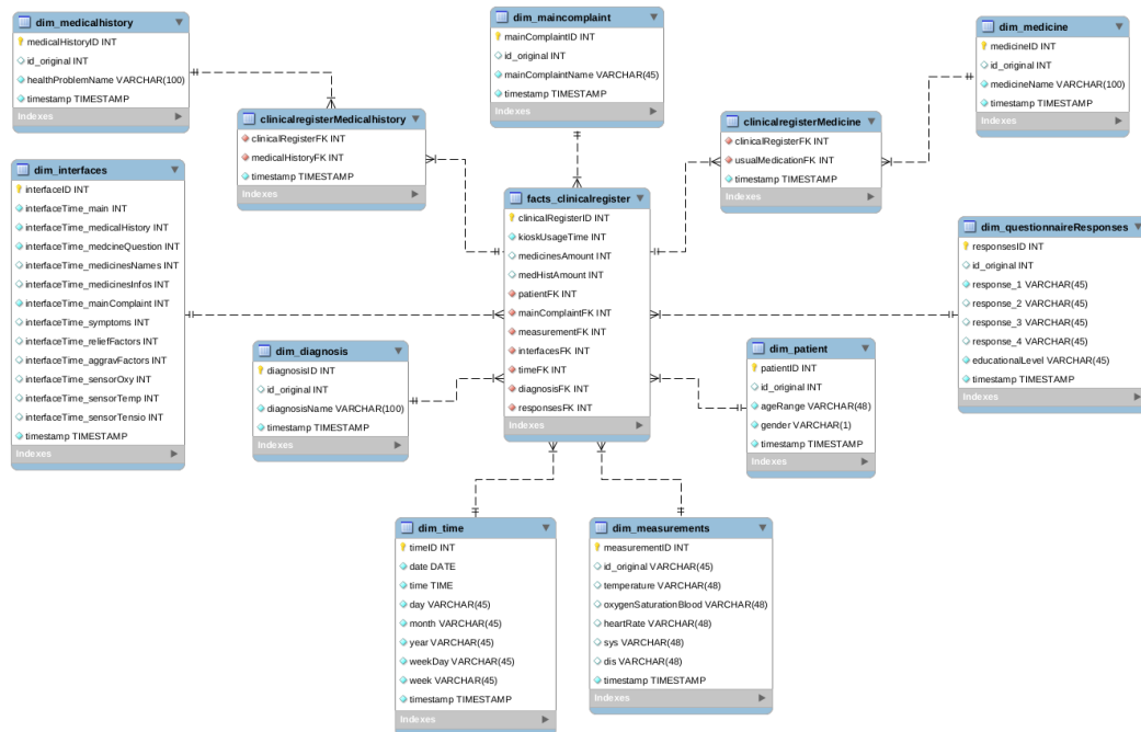
Figure 64: Data warehouse
