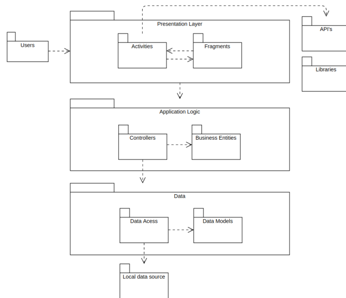
Figure 18: Android architecture
