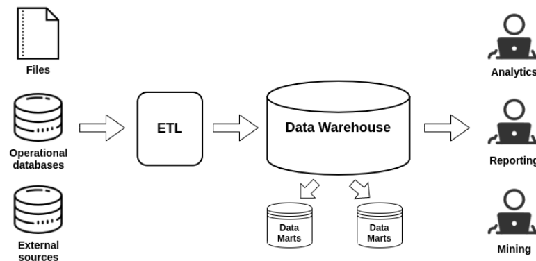
Figure 11: DW architecture, adopted from [27]
