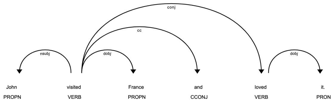
Figure 13: Dependency Tree of a Sentence
