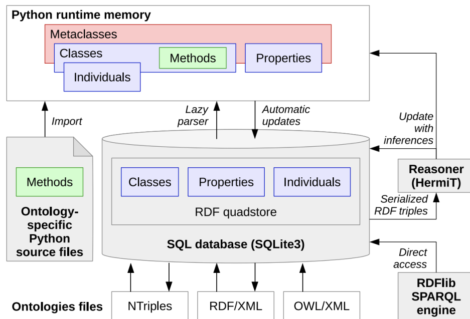
Figure 11: OwlReady Architecture (Lamy, 2017)
