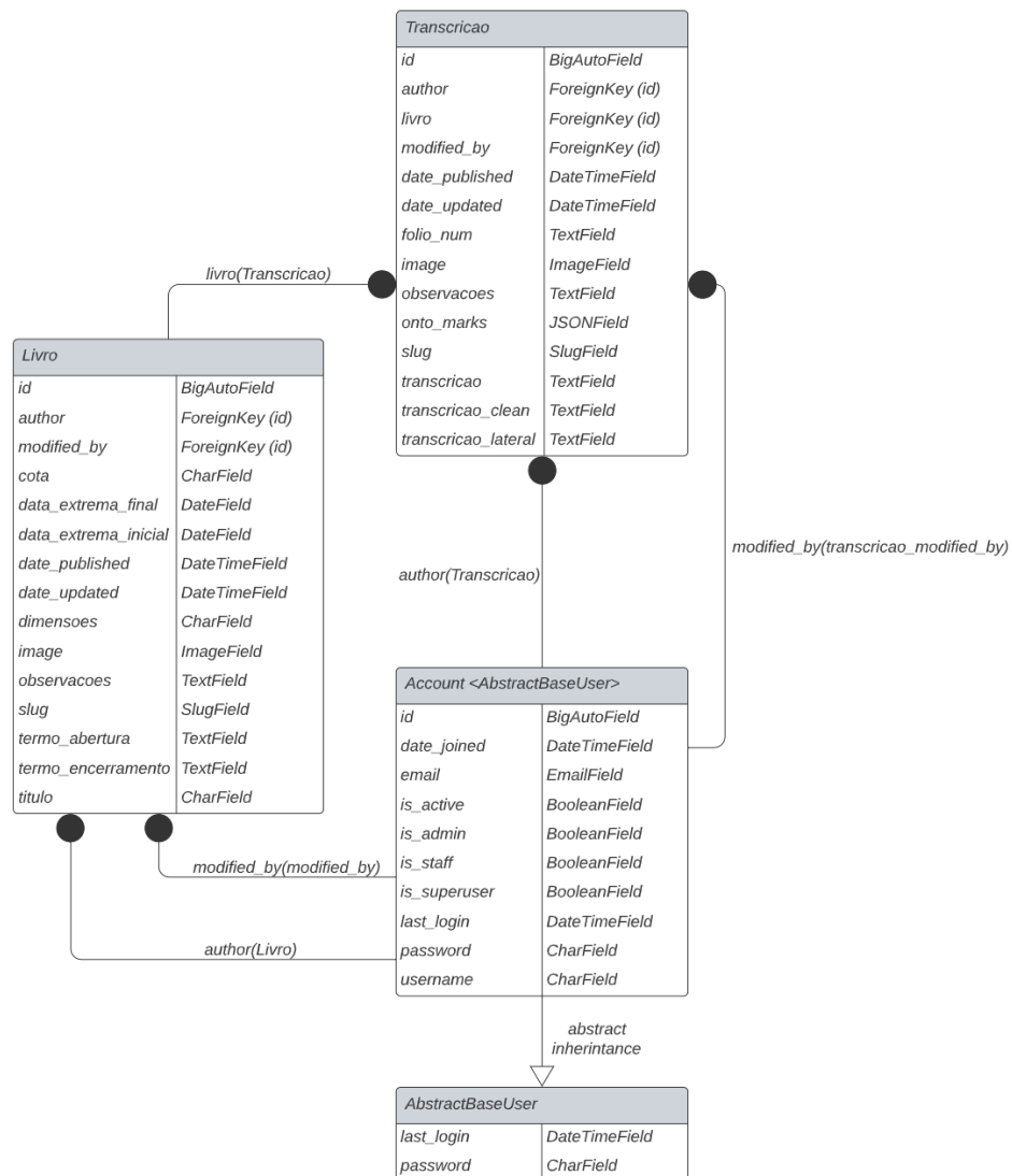
Figure 17: Main Database ERD 1
