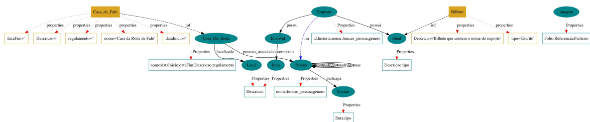
Figure 6: Graphical Ontology Representation
