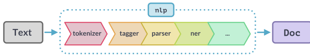
Figure 9: Spacy Pipeline 13
