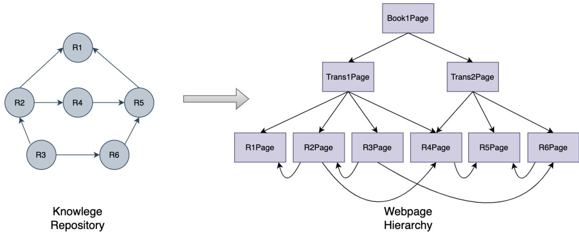
Figure 15: Resources Rendered as HTML Pages
