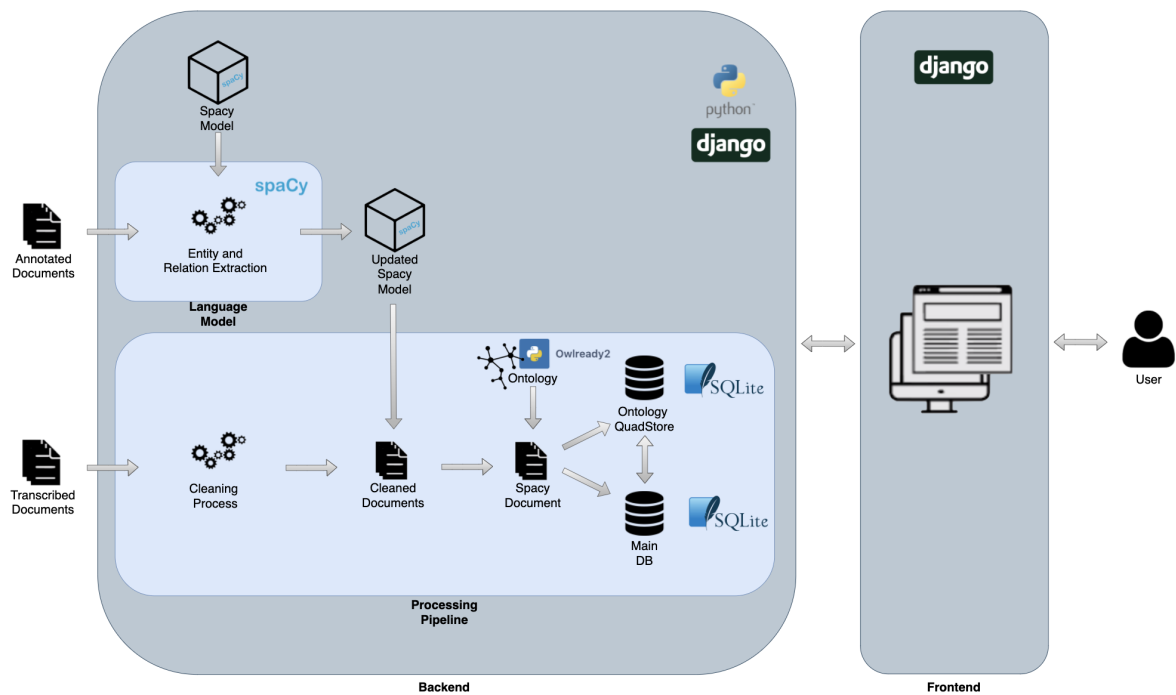
Figure 16: Updated Architecture
