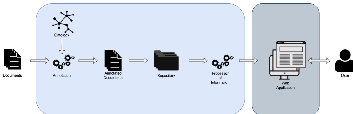
Figure 7: System Architecture
