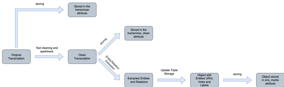
Figure 19: Transcription Processing Pipeline
