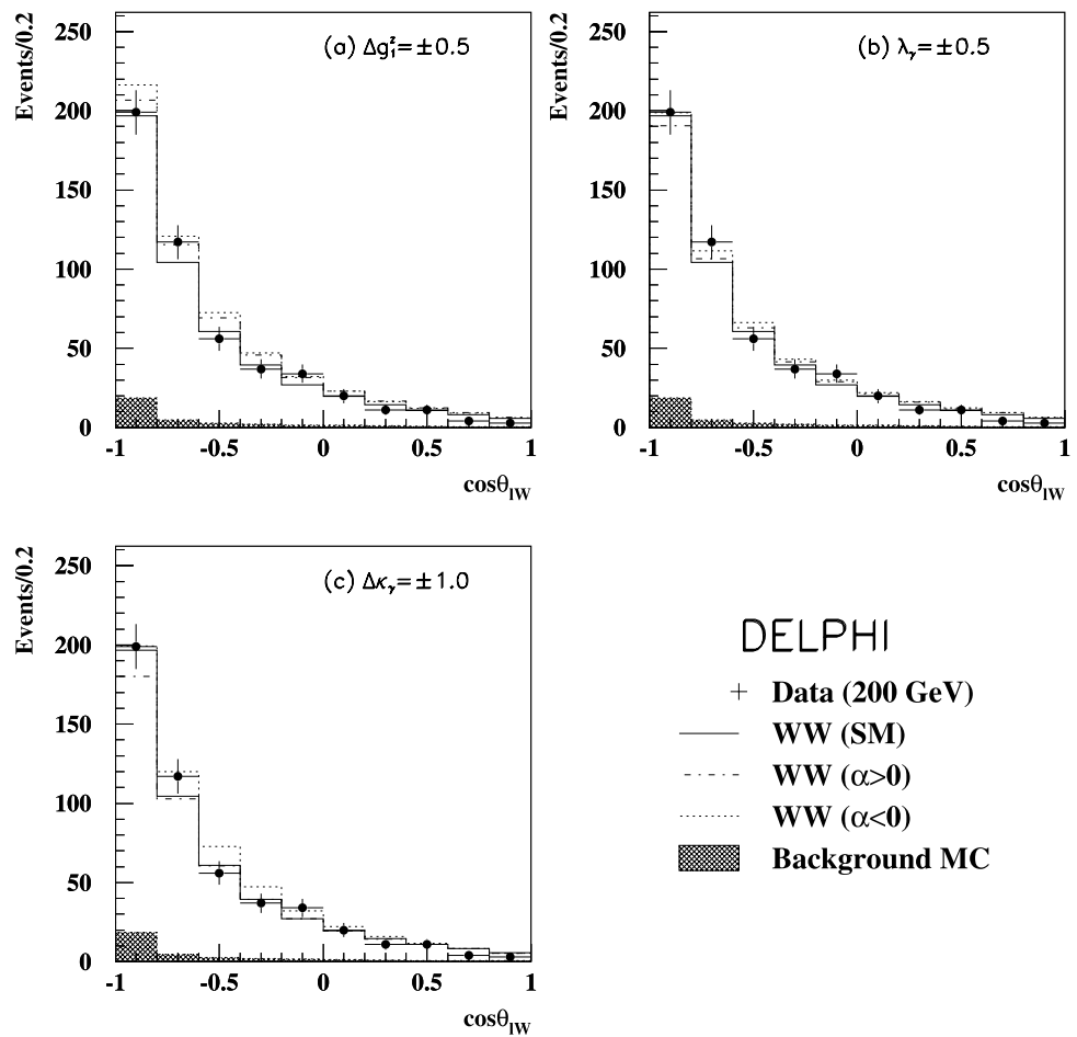
Fig. 8 The distribution of \cos \theta_{lW} , the cosine of the angle between the directions of the lepton and the hadronic W in semi-leptonic events, at a centre-of-mass energy of 200 GeV. All three plots show the data (represented by points ), the Standard Model prediction (the solid line ) and the predicted background (the darker shaded region ). Each plot also shows predictions for non-Standard Model values of a coupling \alpha : in (a), \alpha \equiv \Delta g_1^2 , in (b) \alpha \equiv \lambda_\gamma , and in (c) \alpha \equiv \Delta \kappa_\gamma . The simulated distributions are normalised to the same luminosity as the data
