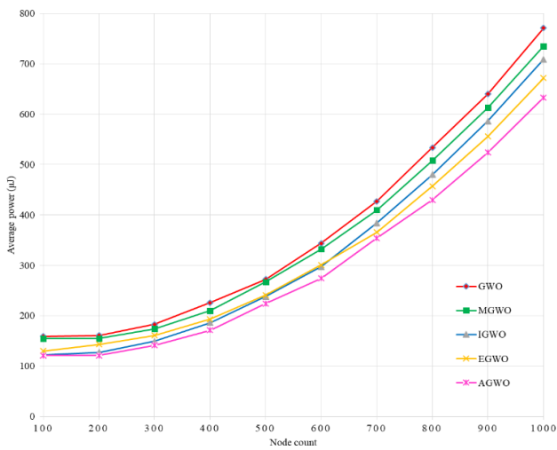
(b) Average power consumption of mobile nodes
