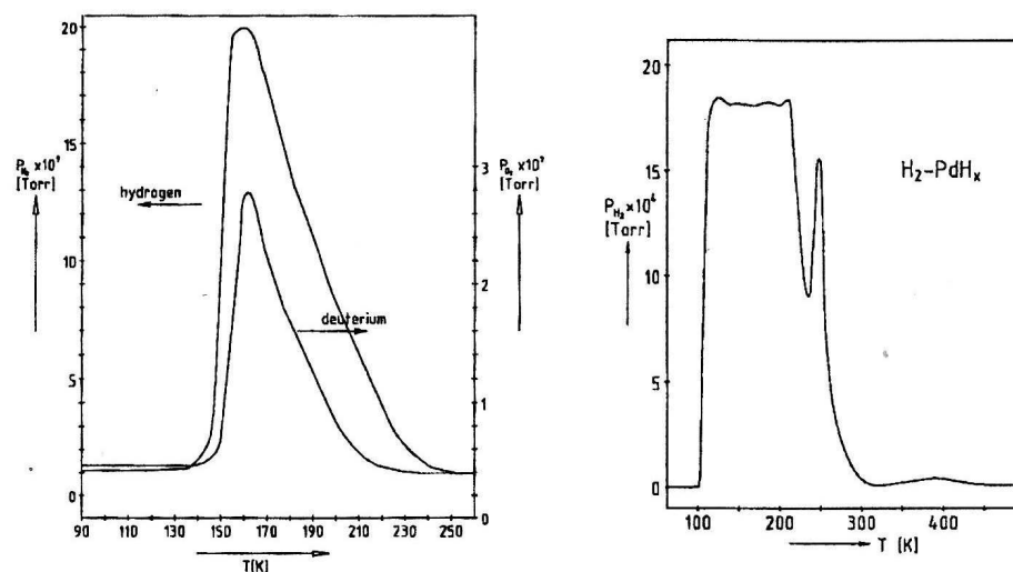
Fig. 4. TDMS spectra obtained from thin Au film as the result of its interaction at 78 K with deuterium (hydrogen) emitted from decomposing thin \text{PdD}_y ( \text{PdH}_x ) films.
