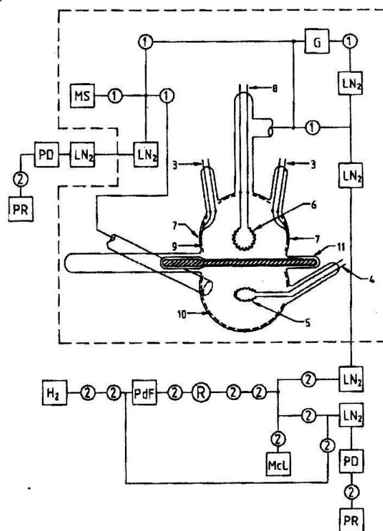
Fig. 1. Schematic diagram of the apparatus. Dotted line indicates the UHV part of the glass system, bakable to 700 K. The markings denote the following units and components: mass spectrometer—(MS), modulated ionization gauge—(G), McLeod mercury manometer—(McL), palladium filter for H_2 ( D_2 )—PdF, calibrated volume for H_2 ( D_2 ) dosing—R, hydrogen (deuterium) container— H_2 , a set of the diffusion mercury pumps (two pumps in series)—PD, rotary pump—PR, liquid nitrogen trap— LN_2 , greaseless Dekker valve—(1), HV tap—(2), tungsten feedthroughs connected to a thin platinum foil semi-melted onto glass for measurements of thin transition metal film resistance (3) and (7), tungsten feedthroughs and heater for thin Au film deposition (4) and (5), tungsten feedthroughs and heater for thin transition metal film deposition (6) and (8), thin transition metal film and thin Au film (9) and (10), damper (11).
