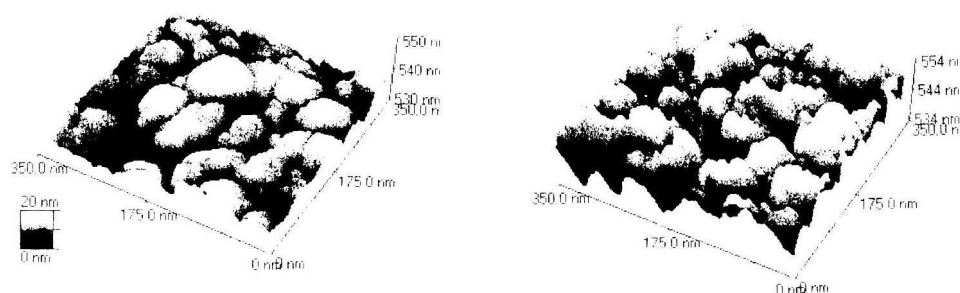
Fig. 2 STM images of a thin Au film (left) and a thin Pd film (right).
