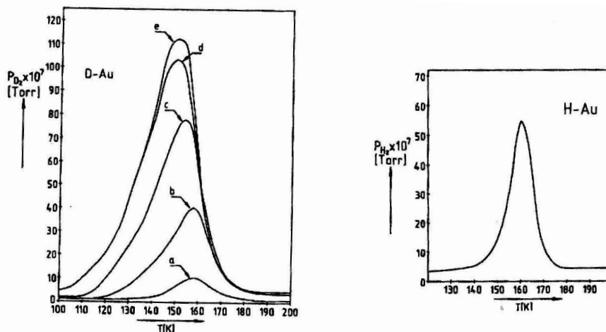
Fig. 3. TDMS spectra for various exposures of thin Au film (maintained at 78 K) to atomic deuterium (hydrogen) generated at 1200 K on tungsten filament at D_2 ( H_2 ) pressure of 6 \times 10^{-3} Torr. The spectra labelled a,b,c and d were obtained as the result of exposure for 1,2,3 and 5 minutes, respectively, at a tungsten filament temperature T_W \approx 1100 K. Spectrum e was obtained for 7 minutes at T_W \approx 1350 K. For comparison, a TD spectrum for hydrogen deposit on thin gold film is also shown (3 min. exposure for atomic hydrogen generated at 1100 K on W filament).
