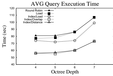
(a) Query Execution Time
