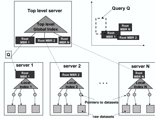
Figure 3. A two-level hierarchical index
