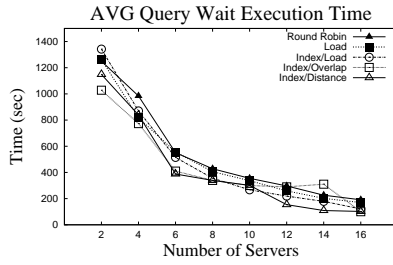
(b) Query Wait + Execution Time
