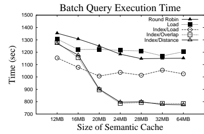
(c) Batch Batch Query Time
