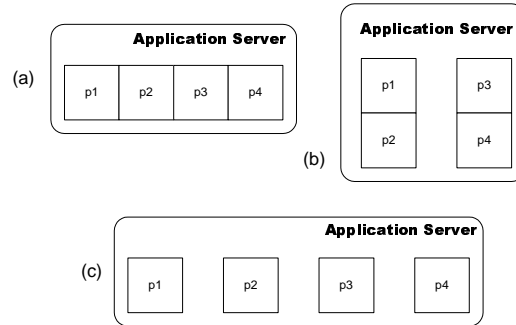
Figure 1. Application Servers with different parallel configurations. (a) shared memory, (b) distributed shared memory, or (c) distributed memory
