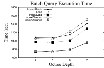
(c) Total Batch Query Time
