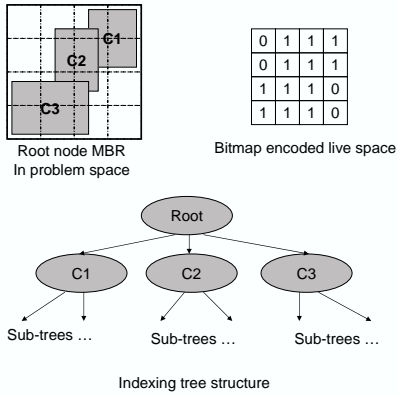
Figure 4. Bitmap live space encoding
