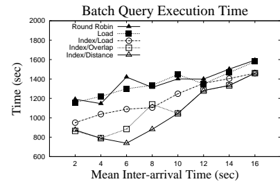
(c) Total Batch Query Time
