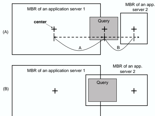
Figure 5. Minimum distance policy
