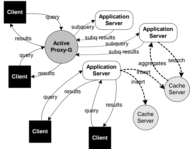
Figure 2. Overview of the MQO middleware
