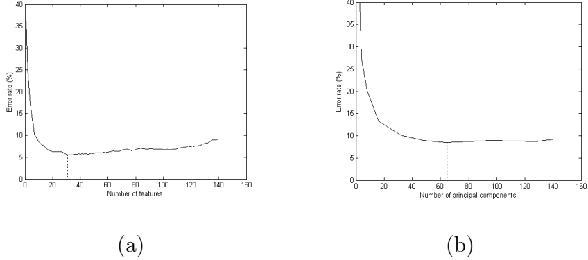
Figure 4.2: Feature analysis. (a) Feature selection: the best classification result is achieved when 31 features are selected. (b) PCA: the best classification result is achieved when 64 principal components are used.
