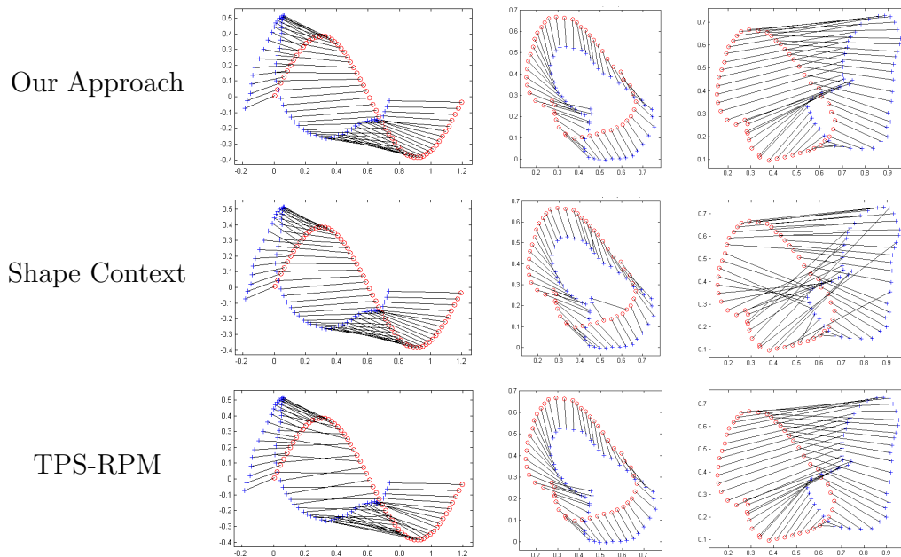
Figure 5.4: Point matching results on open curves (the left column) and closed contours (the middle and right columns). Top row: our approach. Middle row: the shape context algorithm. Bottom row: the TPS-RPM algorithm.
