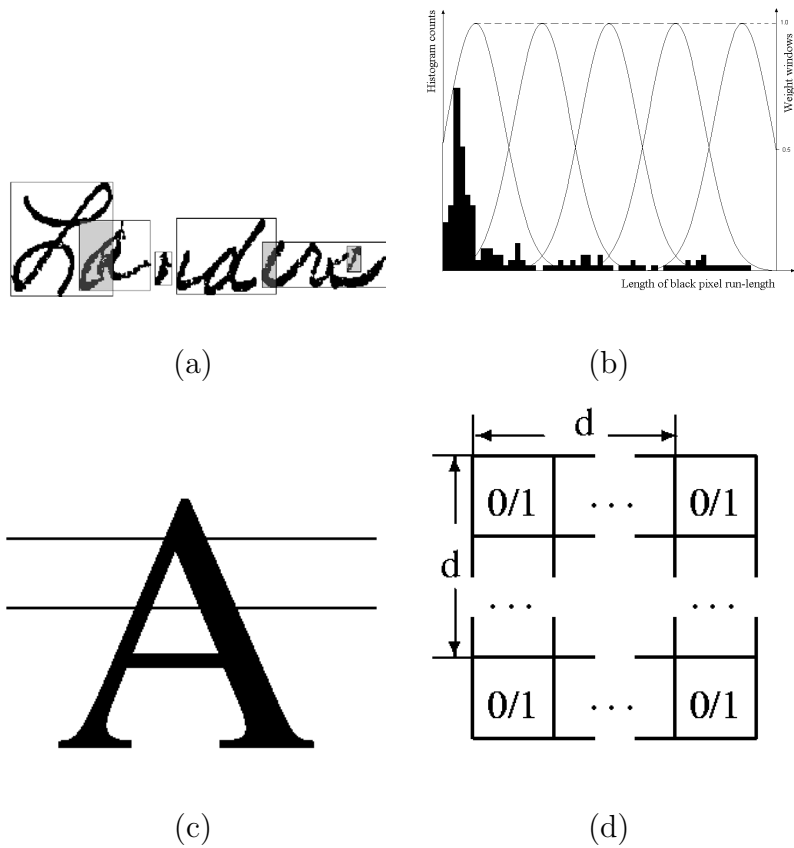
Figure 4.1: Illustration of feature extraction. (a) The overlap area of the connected components inside a pattern unit is extracted as a structural feature. (b) Run-length histogram features. (c) Crossing-count features. The crossing counts of the top and bottom horizontal scan lines are 1 and 2, respectively. (d) Bi-level 2 \times 2 gram features.
