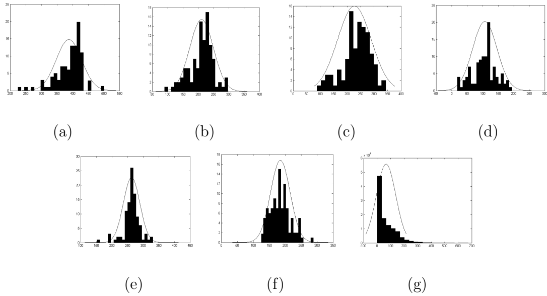
Figure 3.2: The distributions of the observation symbols (horizontal projections) for 100 scanned instances of a bank deposit form. One example of the form is shown in Fig. 3.1a. There are six horizontal lines on the form. (a) to (f) The histograms of the projections of six horizontal lines respectively. (g) The histogram of the projections of the non-line states.
