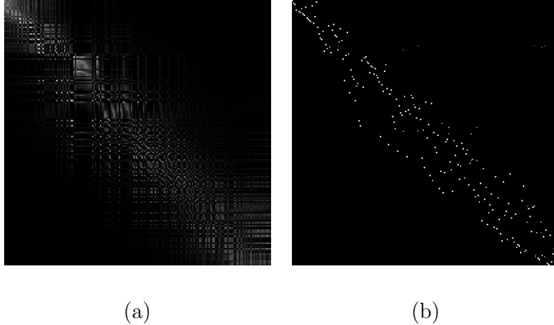
Figure 5.3: Point matching probability matrix P . The matching probabilities to a dummy point are not shown. White represents a high probability. (a) Initial probabilities using the shape context distance. (b) After 300 iterations of relaxation labeling updates.
