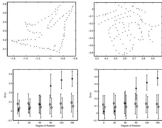
Figure 5.11: Comparison of our results ( \circ ) with the TPS-RPM ( * ) and shape context ( \square ) algorithms under rotation. Left column: the fish shape. Right column: the Chinese character shape. Top row: synthesized samples. Bottom row: mean and variance of errors.
