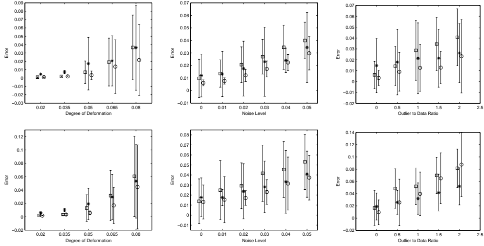
Figure 5.9: Comparison of our results ( \circ ) with the TPS-RPM ( * ) and shape context ( \square ) algorithms on the Chui-Rangarajan synthesized data sets. The error bars indicate the standard deviation of the error over 100 random trials. Top row: the fish shape. Bottom row: the Chinese character shape.
