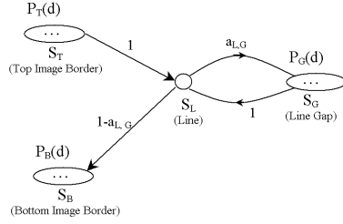
Figure 2.6: A simplified HMM for rule line detection.
