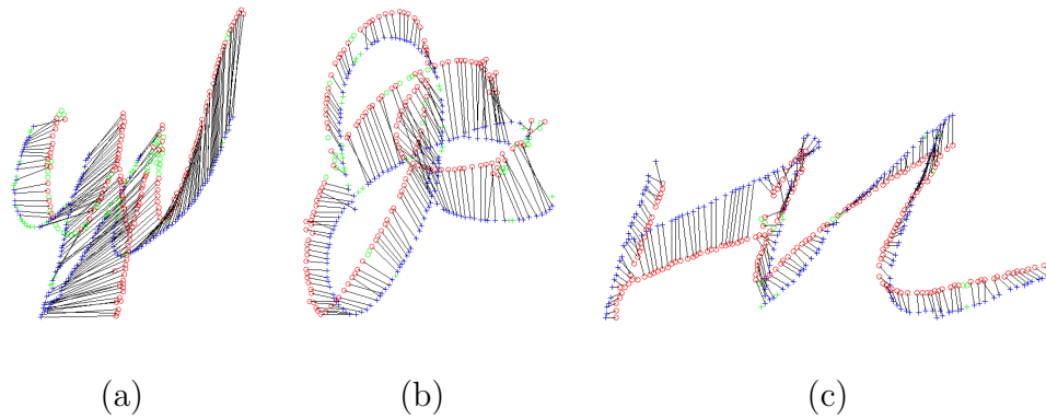
Figure 5.6: More examples of handwriting matching using our approach.
