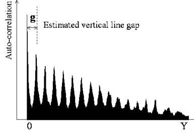
Figure 2.5: Vertical line gap estimation for rule line detection, based on the auto-correlation of the projection profile.
