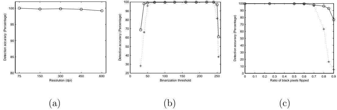
Figure 3.5: Robustness testing. The curves labeled with \circ shows the detection accuracy under the condition where the test set has the same degradation level with the training set. Curves labeled with + are the results when the test set and the training set have different degradation levels. (a) Scanning resolution. (b) Binarization threshold. (c) Synthesized degradation.
