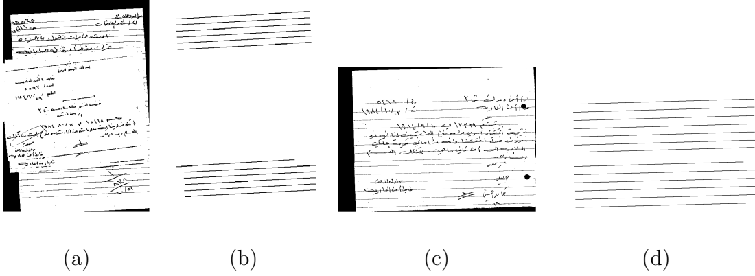
Figure 2.7: Robust test for rule line detection. The image in (a) has enormous observations on the projection profile (several lines missed because two pages are overlapped during scanning). (c) shows a document with enormous line gaps (35 image rows removed manually in the middle). (b) and (d) show the corresponding line detection results.
