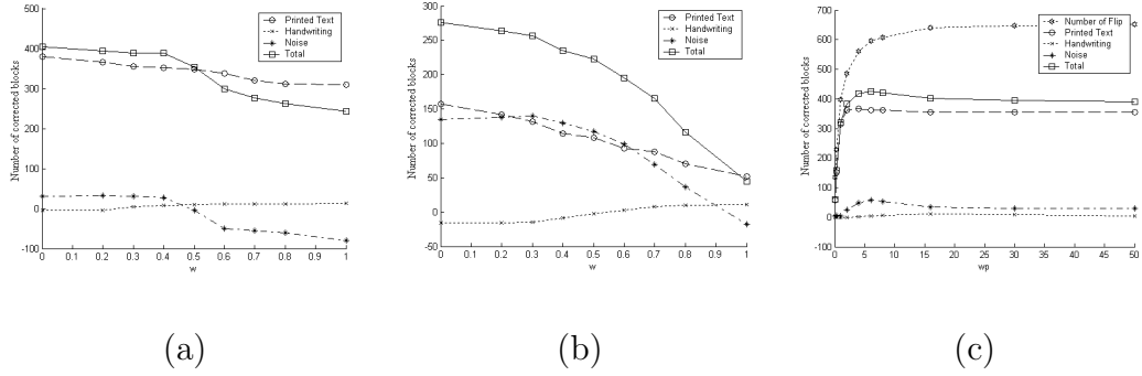
Figure 4.6: MRF-based post-processing. (a) Number of corrected blocks using clique C_p . (b) Number of corrected blocks using clique C_n . (c) Number of corrected blocks using clique C_p and classification confidence.
