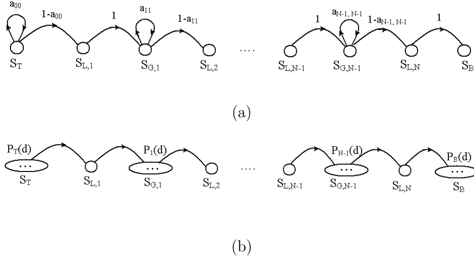
Figure 2.4: HMMs for a projection profile. (a) A standard HMM. (b) An HMM with explicit state duration.
