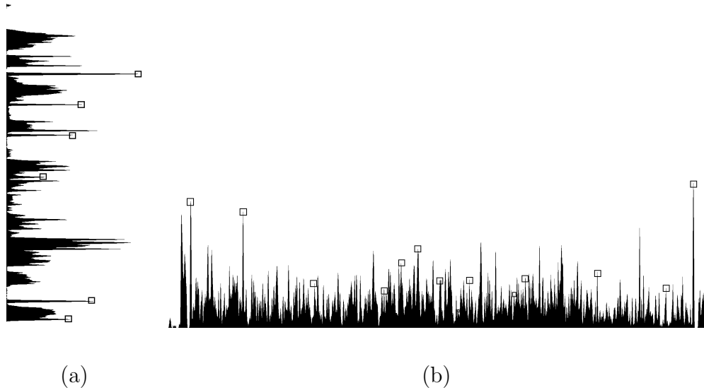
Figure 3.3: The lines detected after decoding the HMMs using the Viterbi algorithm on the horizontal (a) and vertical (b) projection profiles of the bank deposit form. The original form is shown in Fig. 3.1a. The locations picked up by the Viterbi algorithm are labeled with squares.
