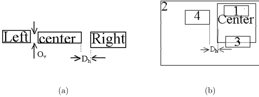
Figure 4.4: Clique definition. (a) C_p for horizontally arranged machine printed words. (b) C_n for noise blocks.
