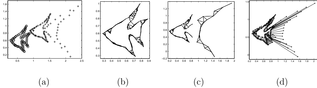
Figure 5.7: A neighborhood definition which is robust under large nonuniform scale changes for different parts of a shape. (a) Point sets of the template (o) and deformed (+) shapes. (b) Template graph with 210 edges. (c) Deformed graph with 196 edges. Among them, 178 (91%) edges also present in the template graph. (d) Point matching result.
