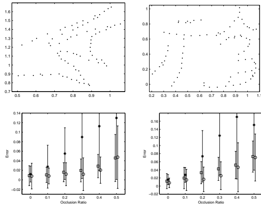
Figure 5.10: Comparison of our results ( \circ ) with the TPS-RPM ( * ) and shape context ( \square ) algorithms under occlusion. Left column: the fish shape. Right column: the Chinese character shape. Top row: synthesized samples. Bottom row: mean and variance of errors.
