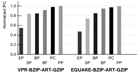
Figure 8: Normalized IPC of the foreground thread when running simultaneously with three background threads. The bars are the same as those in Figure 7.
