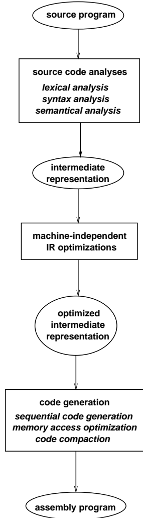
Figure 16: Compilation phases
