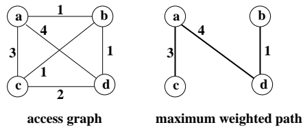
Figure 24: Access graph model and maximum weighted path
