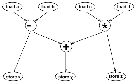
Figure 18: DFG representation of code from fig. 17
