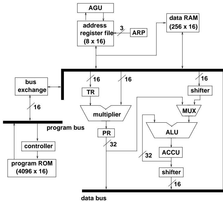
Figure 1: Simplified architecture of Texas Instruments TMS320C25 DSP
