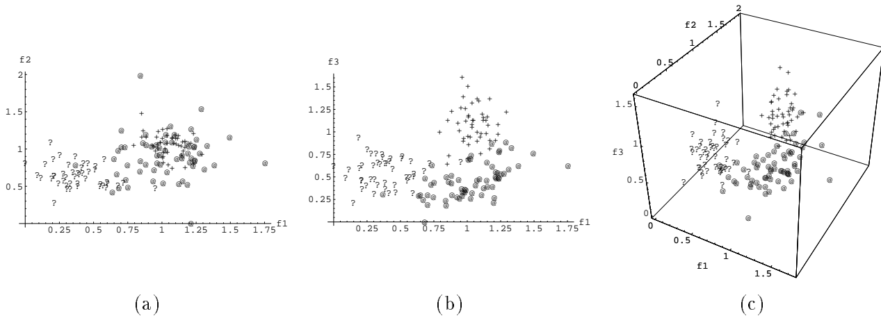
Figure 14: FastMap on WINE dataset (a) k=2 with f_2 vs f_1 , (b) f_3 vs f_1 and (c) k=3
