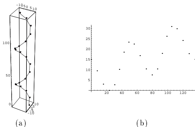
Figure 13: (a) 3-d points on a spiral (SPIRAL dataset) and (b) the result of FastMap , for k=2
