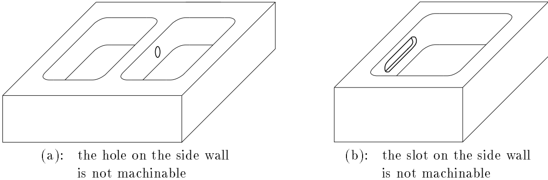
Figure 9: Examples of unmachinable parts, when the set of available machining operations \mathcal{M} is {drilling, end-milling}.
