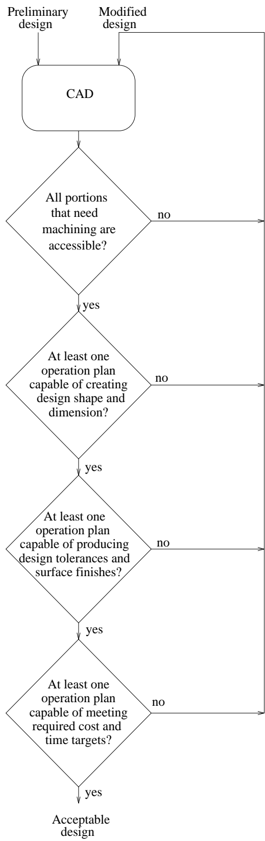
Figure 2: Manufacturability analysis.
