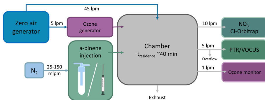
Figure 3. The experimental set-up consists of a continuous stirred-tank reactor (CSTR). Additionally, there are ozone and zero-air generators, an \alpha -pinene injection set-up, an ozone monitor, a nitrate CI-Orbitrap, and a PTR or a Vocus.
