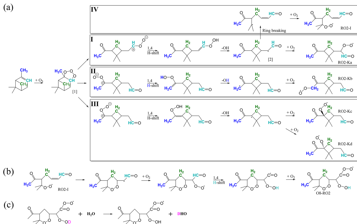
Figure 2. (a) Reaction pathways for \alpha -pinene ozonolysis up until the primary peroxy radical (RO 2 ) from Kurtén et al. (2015) (I–III) and Iyer et al. (2021) (IV). (b) Continued reaction pathway for the IV pathway up to a peroxy radical containing eight oxygen atoms (O 8 –RO 2 ) (Iyer et al., 2021). In panels (a) and (b) the carbon and hydrogen atoms corresponding to deuterated ones in the selectively deuterated precursors are coloured matching the colouring in Fig. 1; i.e. cyan corresponds to the 3 D 1 precursor, green corresponds to the 7 D 2 precursor, and blue corresponds to the 10 D 3 precursor. (c) Deuterium atoms are readily exchanged between HOMs and water vapour if the deuterium is in an –OD or –OOD group, resulting in HOMs without deuterium and semi-heavy water, i.e. a water molecule with one hydrogen atom and one deuterium atom instead of two hydrogen atoms (Rissanen et al., 2014).
