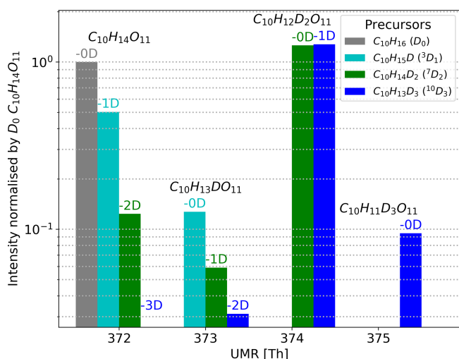
Figure 5. Example spectra using C_{10}H_{14}O_{11} to show resulting HOM signals when using different selectively deuterated precursors. The nitrate cluster of C_{10}H_{14}O_{11} ( C_{10}H_{14}O_{11} \cdot NO_3^- ) is at 372 Th. The colours show which selectively deuterated \alpha -pinene is the precursor, and the values above the bars in matching colour tell how many deuterium atoms the HOMs have lost compared to the precursor. For example, the \alpha -pinene with three deuterium atoms ( ^{10}D_3 , shown in blue) can form up to four different C_{10}H_{14}O_{11} isotopes in the spectrum. However, in the ^{10}D_3 precursor's case there is no signal for C_{10}H_{14}O_{11} without any deuterium atoms ( -3D ).
