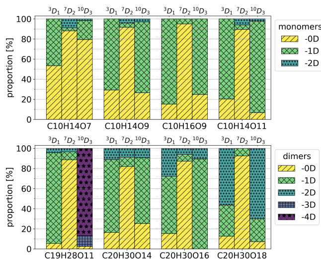
Figure 6. Isotopic distributions of chosen HOMs as proportions of signals using high-concentration C_{high} data. The colours show how many deuterium atoms are lost from the molecule during the formation process. For example, in the case of ^3D_1 precursor and C_{10}H_{14}O_7 compounds, -0D corresponds to C_{10}H_{13}DO_7 and -1D corresponds to C_{10}H_{14}O_7 . The entries for -3D and -4D are excluded from the upper legend as there were no corresponding compounds in the inspected monomers.
