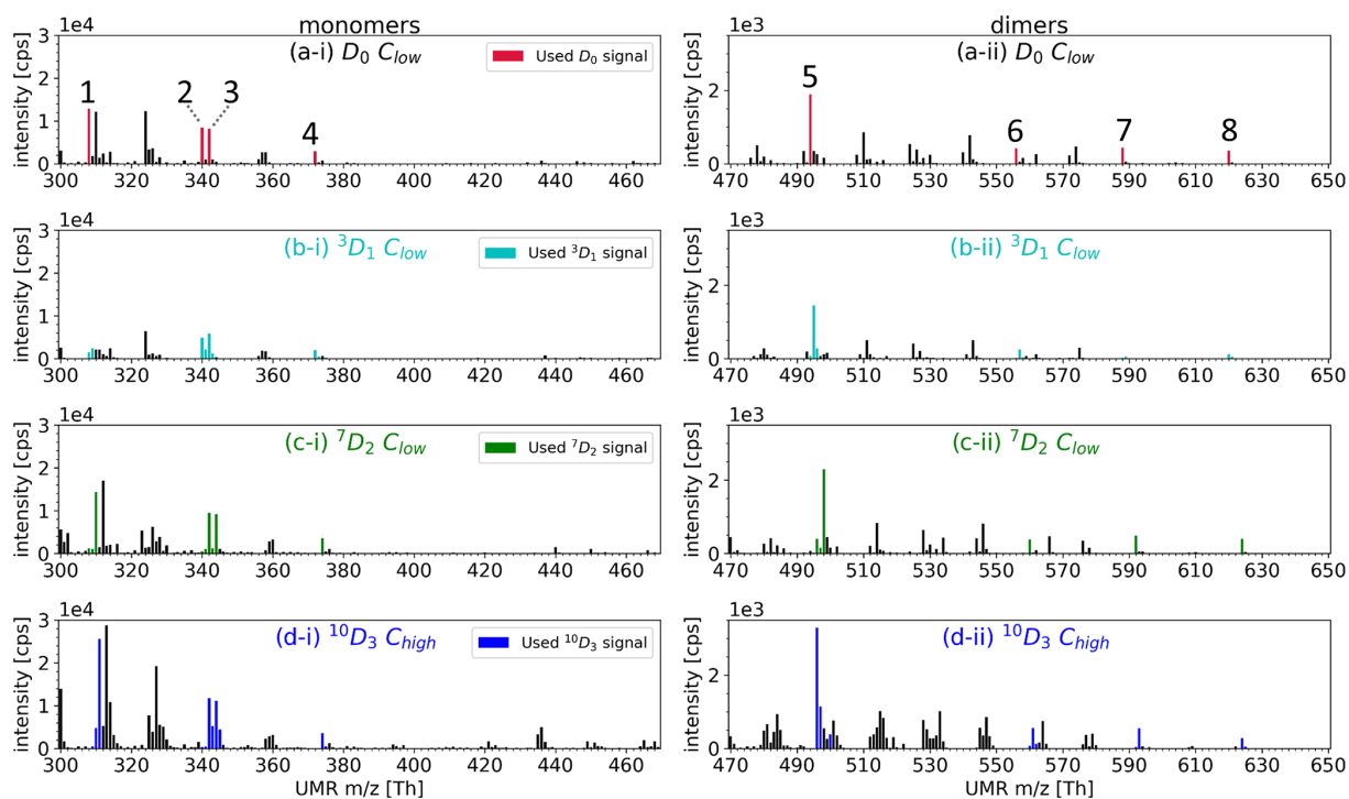
Figure A2. Mass spectra of HOMs from selectively deuterated \alpha -pinene precursors at unit mass resolution. Masses corresponding to HOM signals used on closer inspection are marked with a colour, whereas other peaks in the mass spectra are shown in black. (a-i) and (a-ii) : the closer-inspection compounds are 1. C_{10}H_{14}O_7 , 2. C_{10}H_{14}O_9 , 3. C_{10}H_{16}O_9 , 4. C_{10}H_{14}O_{11} , 5. C_{19}H_{28}O_{11} , 6. C_{20}H_{30}O_{14} , 7. C_{20}H_{30}O_{16} , and 8. C_{20}H_{30}O_{18} . The y scales are different between the monomer and dimer plots.
