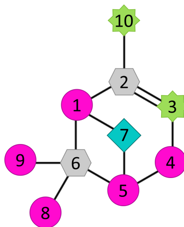
Figure 7. Molecular structure of \alpha -pinene with numbered carbons showing carbons that are active (carbons 3 and 10; green eight-point star) and inactive (carbon 7; light-blue diamond) in the formation process, carbons that were not inspected in this study (carbons 1, 4, 5, 8, and 9; magenta circle), and carbons that cannot be studied using selective deuteration (carbons 2 and 6; grey hexagon).
