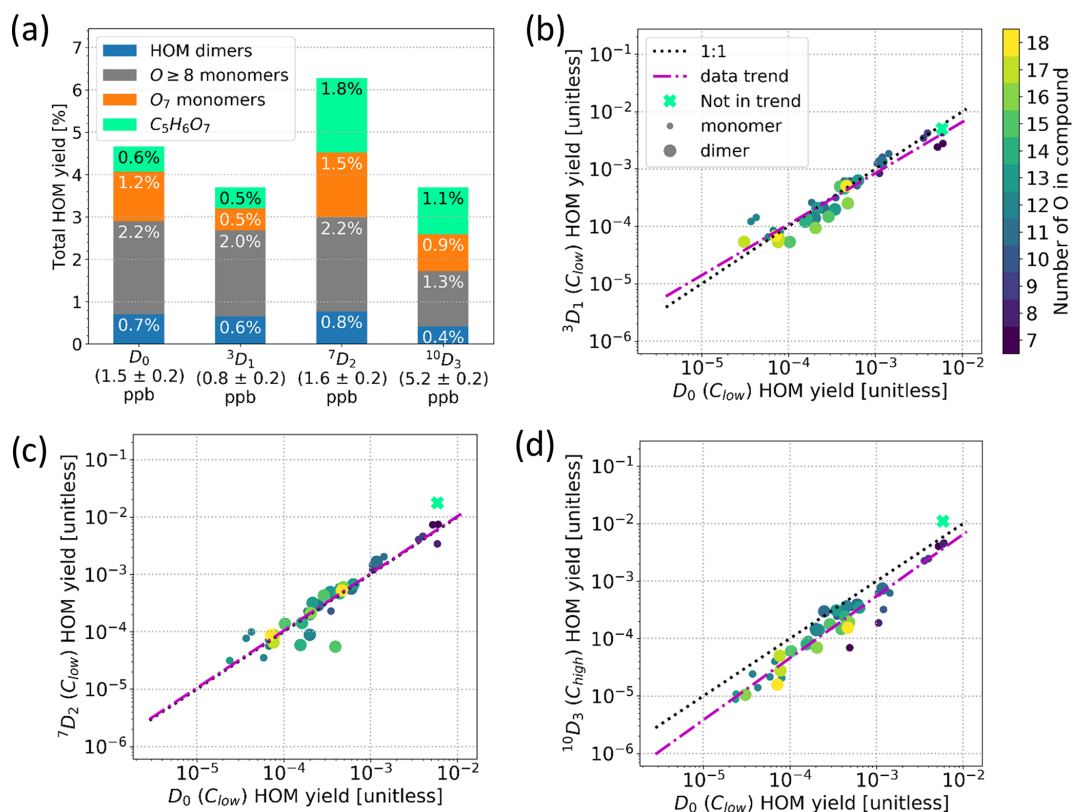
Figure 8. (a) HOM yields for \alpha -pinene samples, where yields for C_5H_6O_7 (mint green), O_7 monomers (orange), O_{8+} monomers (grey), and dimers (blue) are plotted separately. The corresponding precursor names and concentrations are shown on the x axis. (b–d) Comparison of HOM yields compound per compound between the D_0 sample and ^3D_1 sample (b), ^7D_2 sample (c), and ^{10}D_3 sample (d), where the mint green cross corresponds to C_5H_6O_7 and is excluded from the data trend and the colour shows the number of oxygen atoms in the compound. C_{low} and C_{high} refer to the \alpha -pinene concentration of the sample. Note that each point in panels (b)–(d) corresponds to the yield of the sum of all found isotopes per main compound.
