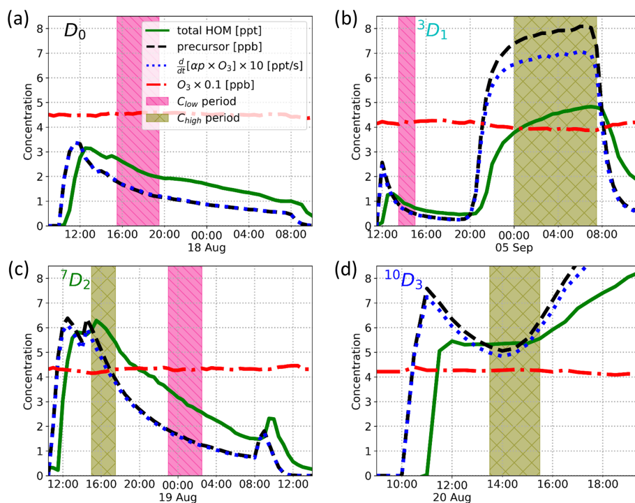
Figure 4. Time series of the experiments showing total HOM concentration (green solid line), precursor concentration (black dashed line), \alpha -pinene ozonolysis rate multiplied by 10 (blue dotted line), and ozone concentration multiplied by 0.1 (red dash-dotted line). Additionally, sample times for a low-concentration sample ( C_{low} ) and a high-concentration sample ( C_{high} ) are shown with a magenta “\” hatched area and an olive cross-hatched area, respectively.
