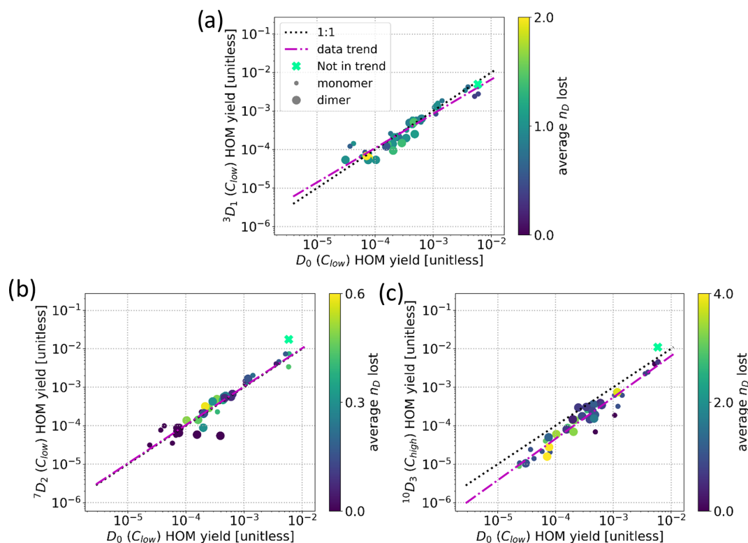
Figure A4. Comparison of HOM yields compound per compound with the number of deuterium atoms lost on average shown with the colour between the D_0 sample and the ^3D_1 sample (a), the ^7D_2 sample (b), and the ^{10}D_3 sample (c), where the mint green cross corresponds to C_5H_6O_7 and is excluded from the data trend. C_{low} and C_{high} refer to the \alpha -pinene concentration of the sample. Note that each point corresponds to the yield of the sum of all found isotopes per main compound.
