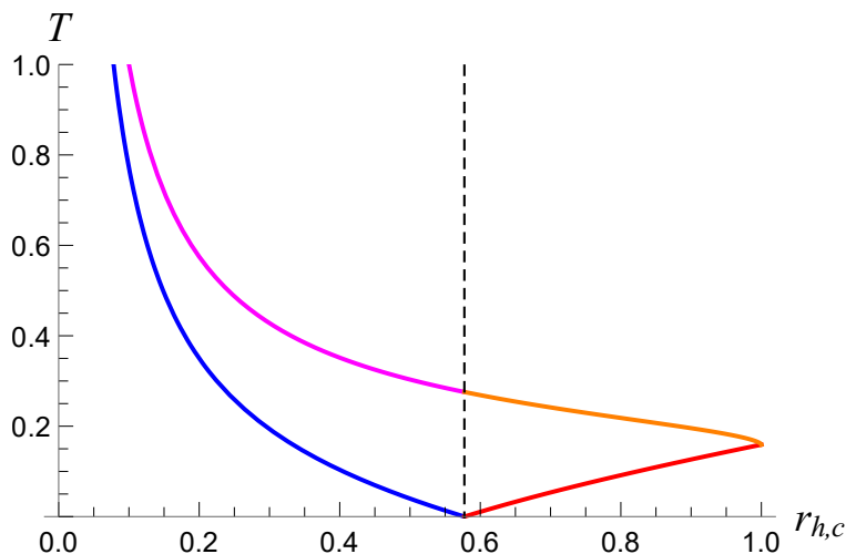
Figure 13. Temperatures of SdS vs. horizon radii r_{h,c} , where we have set d = 4 and L_4 = 1 . The blue and red curves correspond to the temperatures T_h = \kappa_h/2\pi and T_c = \kappa_c/2\pi , respectively, where the surface gravities are defined with respect to the timelike Killing vector \xi = \partial_t . The pink and orange curves show the Bousso-Hawking temperatures \tilde{T}_h = \tilde{\kappa}_h/2\pi and \tilde{T}_c = \tilde{\kappa}_c/2\pi , respectively, where \tilde{\kappa}_{h,c} = \kappa_{h,c}/\sqrt{f(r_0)} given in (B.17). Whereas the former temperatures T_{h,c} vanish for the Nariai black hole with horizon radius r_N = L_4/\sqrt{3} (the dashed line), the latter \tilde{T}_{h,c} are finite and equal to T_N = \sqrt{3}/2\pi L_4 in the Nariai limit.
