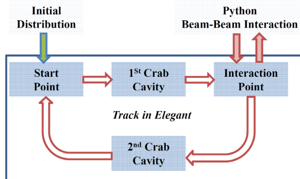
Figure 2: Simulation flow for beam-beam interaction.
