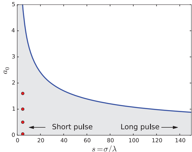
Fig. 2: Region of validity for SENSE shown in gray. Red dots denote the four experimental values for the laser field strength a_0 from the Dresden experiment [24].
