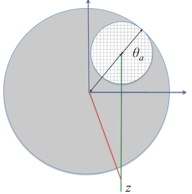
Fig. 3: Geometry of photon scattering. The checkered region represents the physical aperture \theta_a . The shaded region is centered on the point where a scattered photon pierces the plane of the physical aperture. The green line is the z -axis. The red line denotes the path of a scattered photon. The polar coordinates (\cos \theta, \phi) in which the integration is carried out are shown in blue.
