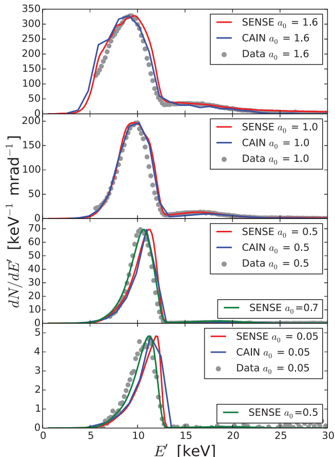
Fig. 4: Simulation of the Dresden experiment [24] data (gray circles) with CAIN (blue line) and with SENSE (red line) for parameters a_0 = 1.6, 1.0, 0.5, 0.05 . Simulations with SENSE use N_s = 4000 particles and circular aperture of \theta_a = 0.004 .
