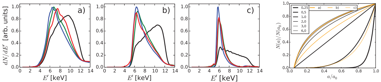
Fig. 5: Panels (a)–(c): simulation of the Dresden experiment [24] for a_0 = 1.6 using SENSE without FM (black lines) and with FM: optimal 1D plane-wave f_{1D} [23] (blue lines), optimal 3D laser pulse f_{3D} [26] (green lines) and RF FM [23] f_{RF} (red lines). The transverse electron beam size is nominal in (a), reduced by \sqrt{10} in (b) and reduced by 10 in (c). Far right: distribution of field strength values a seen by the electron beam for various transverse ratios ( r_x = r_y = 0.25, 0.5, 1, 2, 3, 6 ) in black. Shown in orange are the distributions corresponding to panel (a) with r_x = 3, r_y = 6 , panel (b) with r_x = 1, r_y = 2 , and panel (c) with r_x = 0.3, r_y = 0.6 . A lower cutoff of a > a_{\min} = 0.05 is imposed on the distribution.
