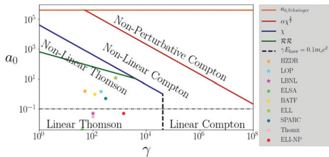
Fig. 1: Regimes of operation for ICS. The red line denotes the boundary between the non-perturbative and perturbative non-linear Compton regimes [8,9]. The blue line indicates the division between Thomson and perturbative Compton scattering. Between the blue and green lines the radiation reaction needs to be taken into account [10–12]. ICS that are in operation are marked as stars and future ICS as dots [13–19].
