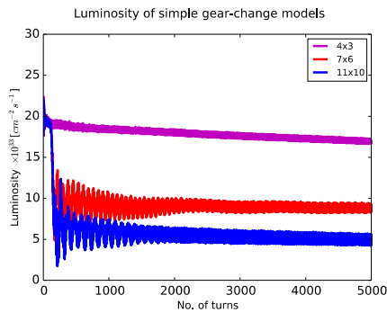
Figure 4: Luminosity vs turn number for simple N_x(N-1) gear-change.
