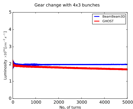
Figure 5: Simplest gear-changing (4x3) luminosity output comparison of BeamBeam3D and GHOST.
