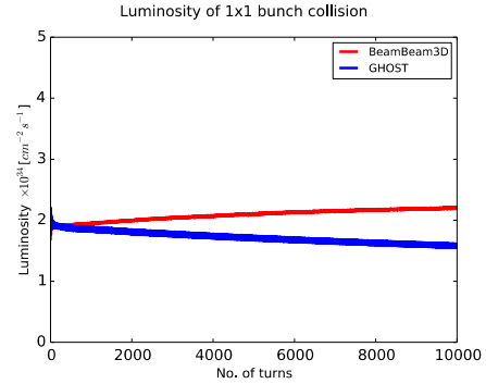
Figure 2: Luminosity output for 1-on-1 collision from BeamBeam3D and GHOST.
