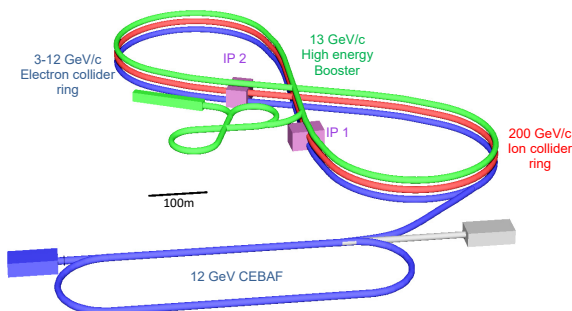
Figure 1: JLEIC layout for 200 GeV ion ring.
