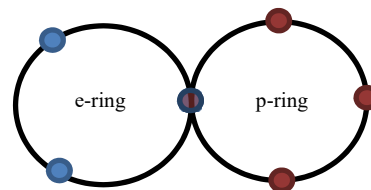
Figure 3: Schematic for 4 \times 3 bunch collision.
