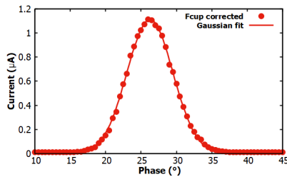
Figure 3: Chopper phase scan for 4 \mu\text{A} beam at 499 MHz with prebuncher OFF.
