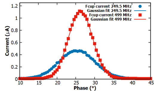
Figure 4: Chopper phase scans for two laser frequencies with prebuncher OFF. The length of the bunch is about 42.50 \pm 0.22 ps FWHM for 499 MHz drive frequency and about 63.83 \pm 0.27 ps FWHM for 249.5 MHz drive frequency.
