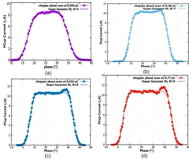
Figure 5: Longitudinal bunch profile measurements at the chopper for (a) 0.096 pC at 499 MHz, (b) 0.48 pC at 249.5 MHz, (c) 0.656 pC at 249.5 MHz, and (d) 0.77 pC at 249.5 MHz.
