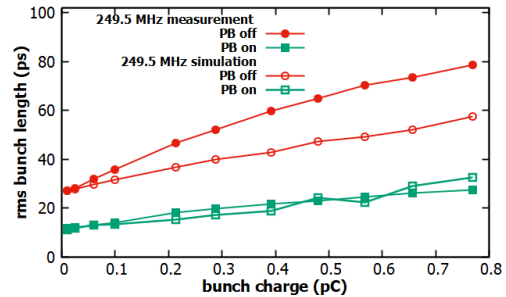
Figure 7: Bunch length at the Chopper for 249.5 MHz laser drive frequency.
