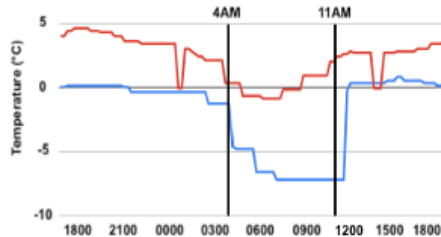
Figure 9. Air temperature (blue) and the temperature inside the box (red) as MARCo survives a 24-hour test on a cloudy day. Monitoring the box or the battery temperature is crucial as all battery capacities drop drastically at low temperatures. The graph shows the battery environment reaches its lowest temperature between 4 AM and 11 AM. Based on this, it is best for the system to perform minimal tasks between 4 AM and 11 AM.
