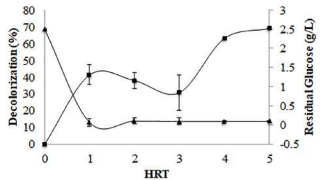
Figure 4 Relationship between residual glucose (▲) and color removal (■) at the outlet
