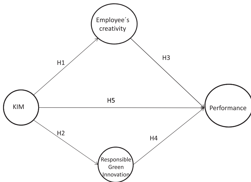
FIGURE 1 Theoretical model
