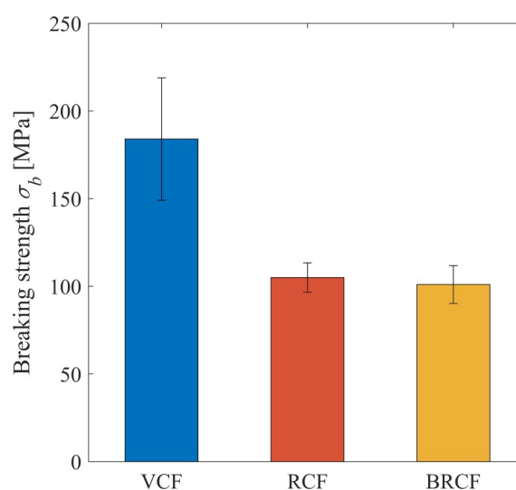
Figure 3. Breaking strength \sigma_b for virgin carbon fibre (VCF), recycled carbon fibre (RCF) and blended recycled carbon fibre (BRCF) ( n = 5 ).
