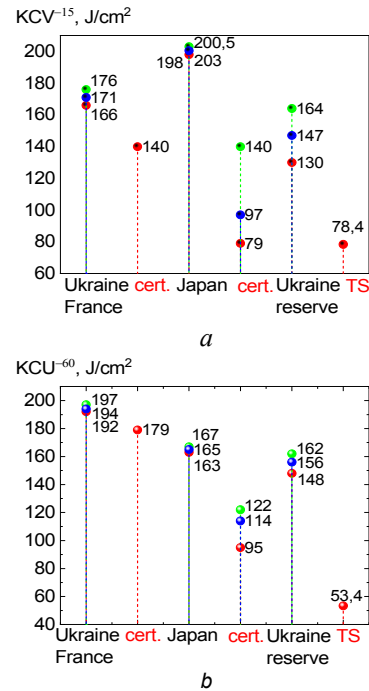
Figure 5. Impact viscosity of the base metal of tested pipes at different temperatures KCV^{-15} (a) and KCU^{-60} (b).
