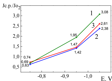
Figure 10. Change in the ratio j_{c.p.} / j_{O_2} defined for X70 pipe steel: 1 – after 20 years of operation, steel manufacturer France, pipe manufacturer Ukraine; 2 – after 20 years of operation, steel and pipe manufacturer Japan; 3 – after 20 years of storage, the steel producer is not established, pipe manufacturer in Ukraine.
