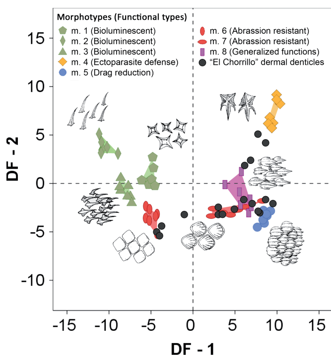
Figure 2. Canonical Variate Analyses results showing the discriminant punctuations of “El Chorrillo” dermal denticles. Results are plotted based on the first two discriminant functions (DF). The analysis was performed taking eight dermal denticle morphotypes (m. 1 - m. 8, corresponding to five functional types) as defined groups and ten size-free variables of the crown surface as discriminant variables. Modified from Ferrón et al. (2018).
