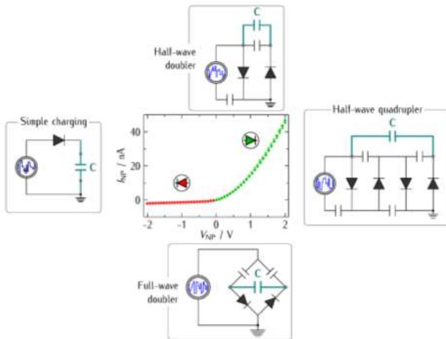
Figure 2. Four practical realizations [13-15] of hybrid circuits based on nanofluidic diodes and load capacitors. The electrical rectification shown by the current ( I )–potential ( V ) curve of a single nanofluidic diode (center) allows the conversion of white noise input potentials into net currents. [10] These currents permit to charge a load capacitor (simple charging process). The hybrid networks with the half-wave (HW) doubler, full-wave (FW) doubler, and FW quadrupler shown schematically permit to scale up the energy conversion.
