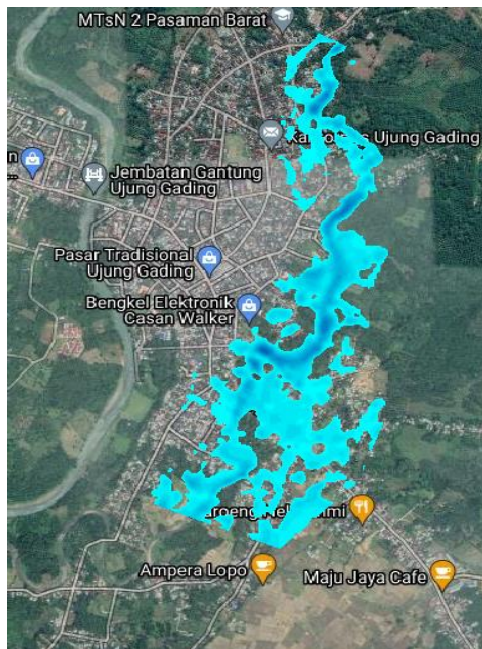
Figure 12. River Overflow Area 25 year Return Period.
