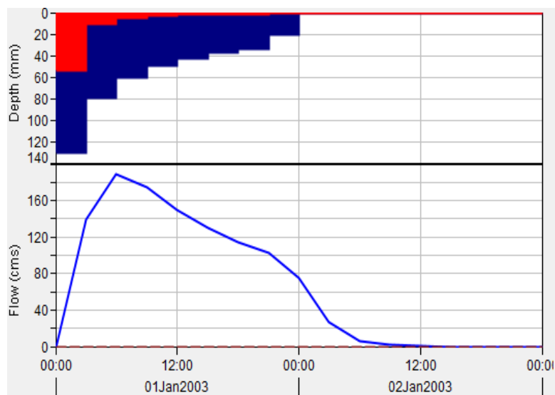
Figure 4. Graph of Flood Discharge for 25 Years Return Period
