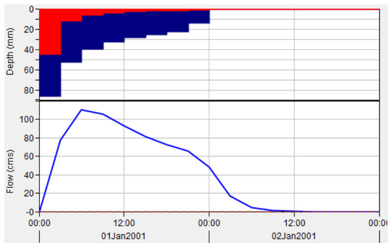
Figure 2. Graph of Flood Discharge for 5 Years Return Period
