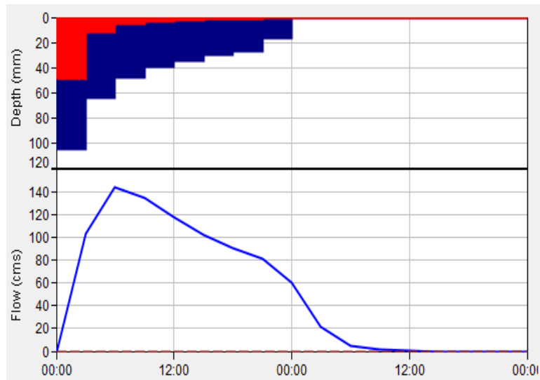
Figure 3. Graph of Flood Discharge for 10 Years Return Period
