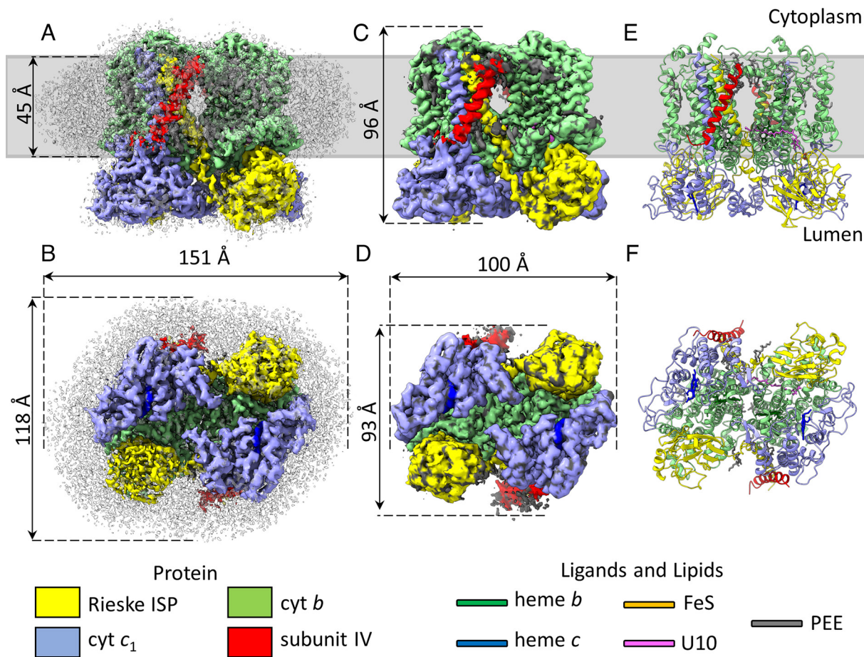
Fig. 2. Color-coded cryo-EM map and refined model for the R. sphaeroides four-subunit cyt bc_1 complex. (A and B) Postprocessed map viewed in the plane of the membrane (A) and from the luminal face (B). (C and D) The map after local sharpening, which removed the disordered density of the nanodisc and improved interpretability for low-resolution portions of the map. (E and F) The refined model with the protein in cartoon representation, and ligands and lipids in stick representation. The gray bar in panels (A, C, and E) indicates the approximate position of the membrane. U10 = ubiquinone-10 and PEE = 1,2-dioleoyl-sn-glycerol-3-phosphoethanolamine.
