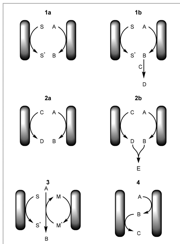
Fig. 7 Types of reactions in electrochemical synthesis; S: solvent, S * : solvent degradation product; A and C: reagents; B, D and E: product; M: mediator or catalyst, M * : activated mediator or catalyst.
