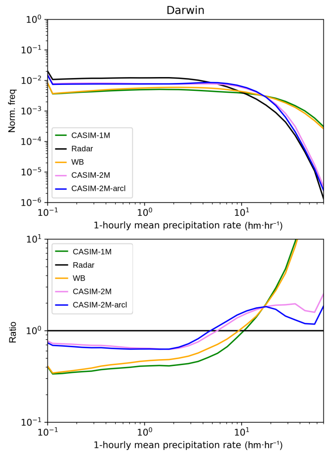
FIGURE 4 Darwin case-study histograms of precipitation rate for the models and the radar-derived surface precipitation rate (top) and ratio of models to radar precipitation rate (bottom). Only bins with greater than 30 observations are shown. CASIM: Cloud AeroSol Interacting Microphysics; WB: Wilson–Ballard
