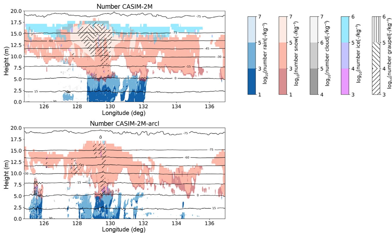
FIGURE 14 Darwin tropical storm example. Cross-section of grid-box-mean number mixing ratios for CASIM-2M and CASIM-2M-arcl from T + 24 output of the Darwin simulation for 1200 UTC March 5, 2017
