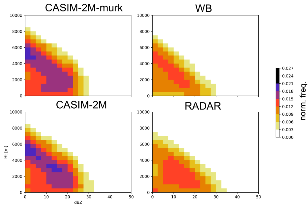
FIGURE 5 United Kingdom Variable grid two-dimensional normalised histograms (contoured frequency by altitude diagrams) of radar reflectivity and height. The normalisation includes values <0 dBZ. CASIM: Cloud AeroSol Interacting Microphysics; WB: Wilson–Ballard
