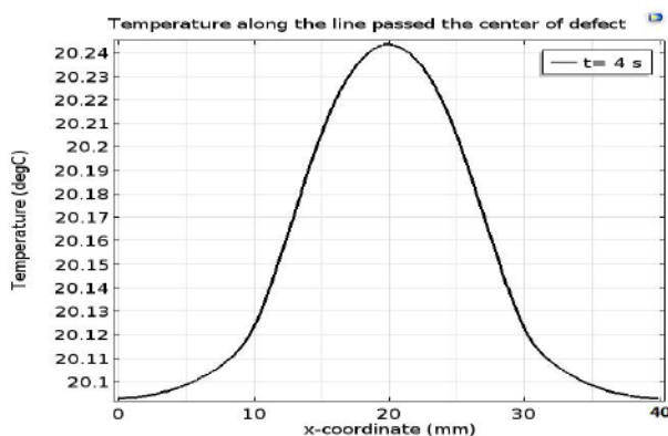
Fig. 8 Temperature profile along the line y = 125 mm, z = 3 mm and 0 \text{ mm} \leq x \leq 40 \text{ mm} crossing the defect zone
