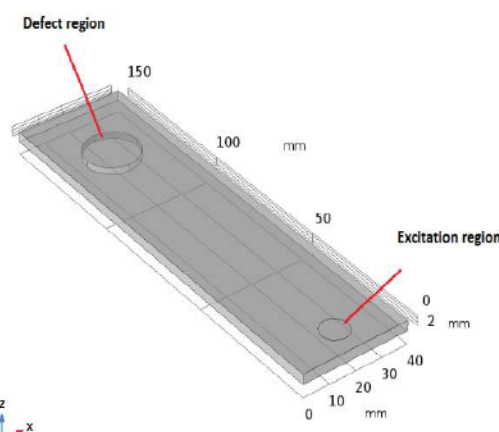
Fig. 1 Geometry of the simulated aluminum part showing the FBH defect and the excitation regions
