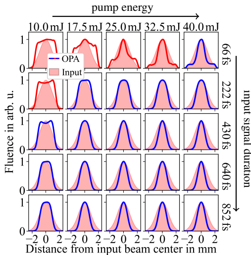
Figure 3: Simulated, normalized fluence lineouts of the signal after uOPA at an output energy of 1 mJ (solid lines, referred to as 'OPA' in the legend) and of the input distribution (red shaded area, referred to as 'input' in the legend). Blue lines indicate that 1 mJ of output energy was achievable in this setup. If this was not the case, red lines represent the distribution after the maximum propagation distance of 1.5 mm. The input parameters for this simulation are a pump-to-signal angle of -2.25^\circ and a seed energy of 1 \mu\text{J} . The pump energy and signal duration has been varied according to the titles on the top and right, respectively. The beam sizes were not changed compared to the simulation in Fig. 1.
