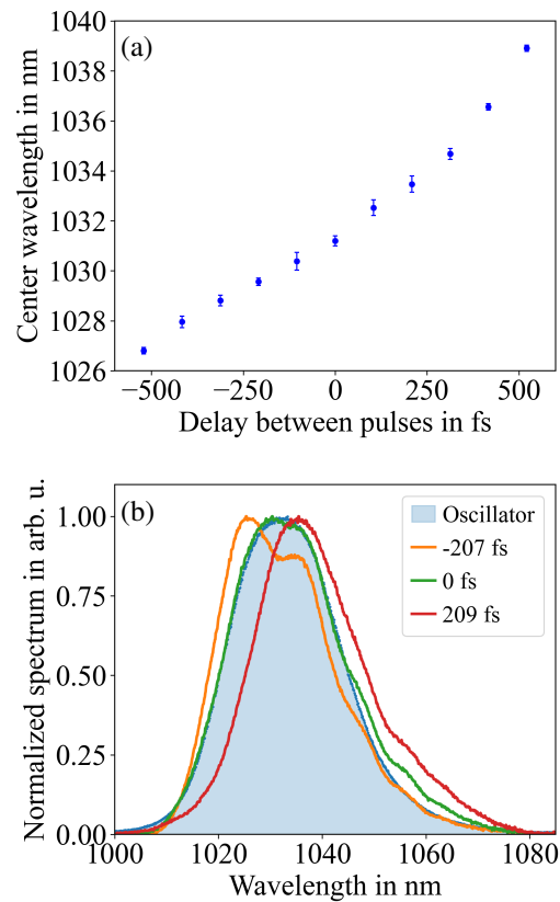
Figure 12: Average shift of the spectral center of gravity by delay (a) and spectra of the uOPA output in dependency of the delay between pump and seed (b). The blue-shaded region marks the original seed spectrum of the oscillator.
