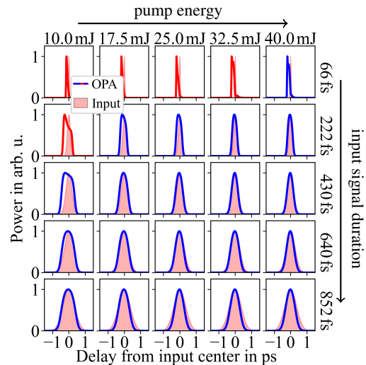
Figure 4: Simulated, normalized power, integrated over the spatial profile of the signal after uOPA at an output energy of 1 mJ (solid lines, referred to as 'OPA' in the legend) and of the input distribution (red shaded area, referred to as 'input' in the legend). Blue lines indicate that 1 mJ of output energy was achievable in this setup. If this was not the case, red lines represent the distribution after the maximum propagation distance of 1.5 mm. Same simulation parameters as in Fig. 3
