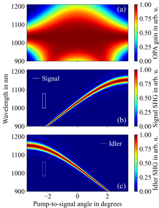
Figure 2: (a): Calculated normalized parametric gain of the uOPA for a pump at 515 nm with an intensity of 80 GW/cm 2 and a 1 mm thick BBO crystal. The pump-to-signal angle defines the phase-matching angle between the signal at 1034 nm and the crystal axis. For this angle, we calculated the normalized SHG-efficiency at every wavelength for the signal (b) and the idler (c). The white dashed and dotted lines mark the spectral range of the signal and idler input wavelengths for a pump-to-signal angle of -2.25^\circ \pm 0.1^\circ . The calculations did not include pump depletion.
