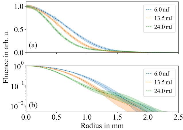
Figure 9: Exemplary radial lineouts of the beam after the second uOPA stage at different pump energies of 6 mJ 13.5 mJ and 24 mJ. (a): linear scale. (b): log-scale.
