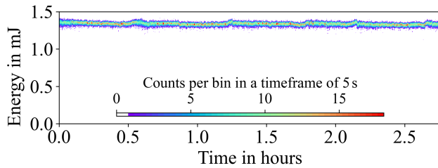
Figure 13: Stability measurement of the uOPA system over approximately three hours in a test laboratory. The colorbar represents the distribution of the energy over a 5 s timespan to visualize the short-term stability. The mean energy of this measurement was 1.3 mJ
