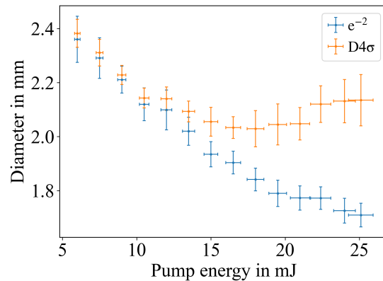
Figure 8: Beam diameters after amplification in the second uOPA-stage, measured at a threshold of \exp(-2) (blue data) and via second moment of the distribution (orange data).
