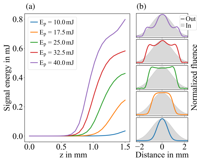
Figure 1: Simulation of a Beta Barium Borate (BBO) based single-stage uOPA. (a): Signal energy of the uOPA as a function of the crystal length and the pump input energy. (b): Comparison of the normalized fluence lineouts after OPA (solid line) with the input distribution (shaded area) at 1.5 mm. The colors correspond to the legend entries in (a). Input parameters of the signal are t = 66 fs (FWHM, Gaussian), w = 1.8 mm (Gaussian) and E = 1 nJ. Input parameters of the pump are t = 1.5 ps (FWHM, Gaussian), w = 2.14 mm (Gaussian).
