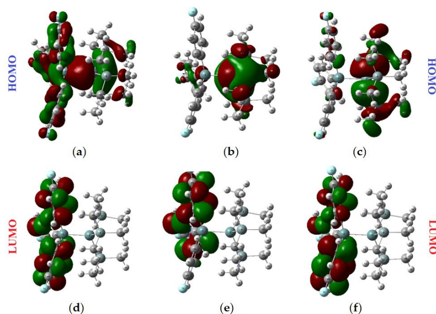
Figure 3. Graphical representation of the frontier orbitals of (\text{Me}_3\text{Si})_3\text{Ge-Ge}(\text{C}_6\text{H}_4\text{F-}p)_3 (2): (a) HOMO; (b) HOMO-1; (c) HOMO-2; (d) LUMO; (e) LUMO+1; (f) LUMO+2.
